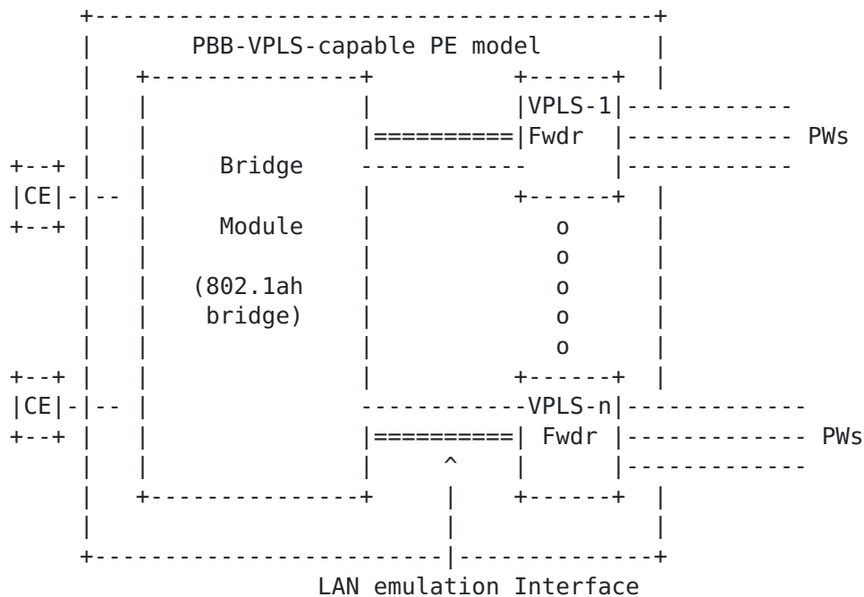
Figure 2: PBB-VPLS capable PE Model
