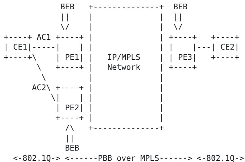
Figure 1: PBB-EVPN Network
