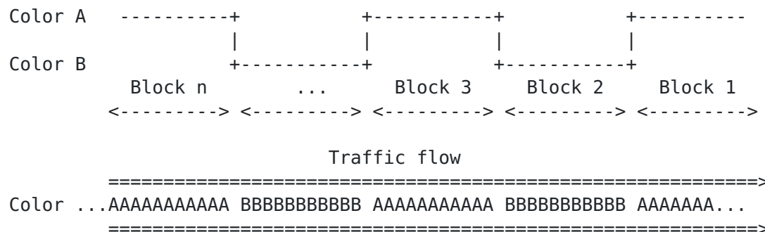
Figure 3: Computation of link packet loss
