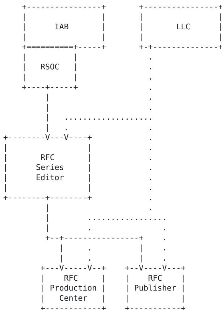
Authority Structure of the RFC Series
