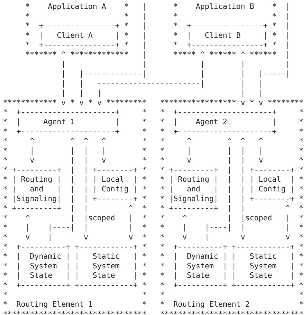
Figure 1: Architecture of I2RS clients and agents
