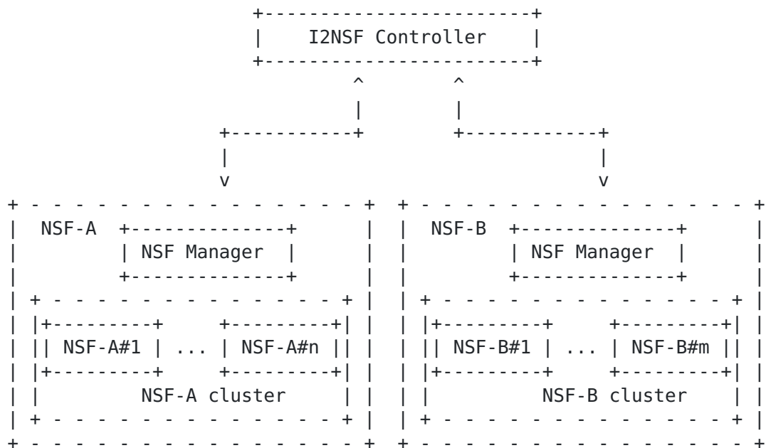
Figure 2: Cluster of NSF Instantiations Management
