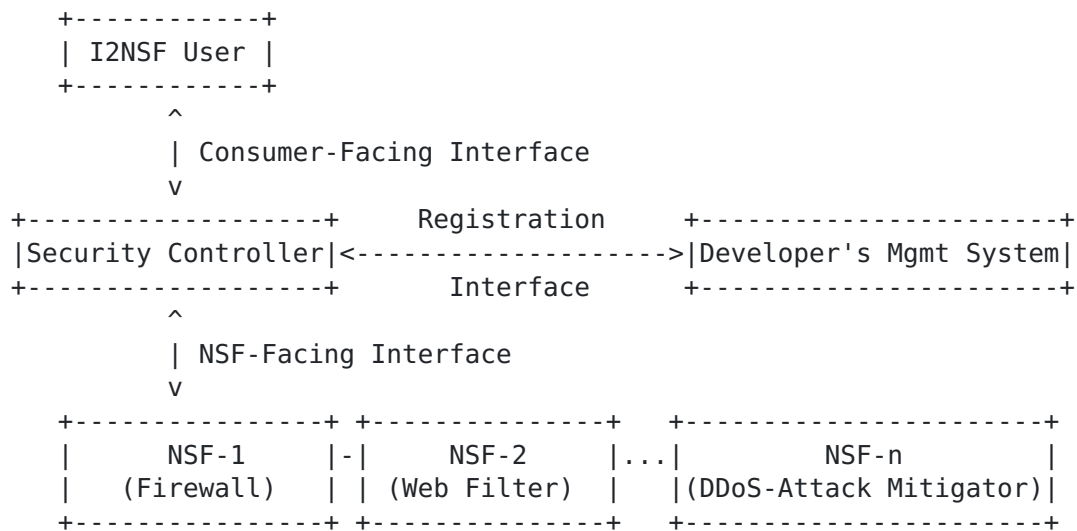
Figure 1: I2NSF Framework
