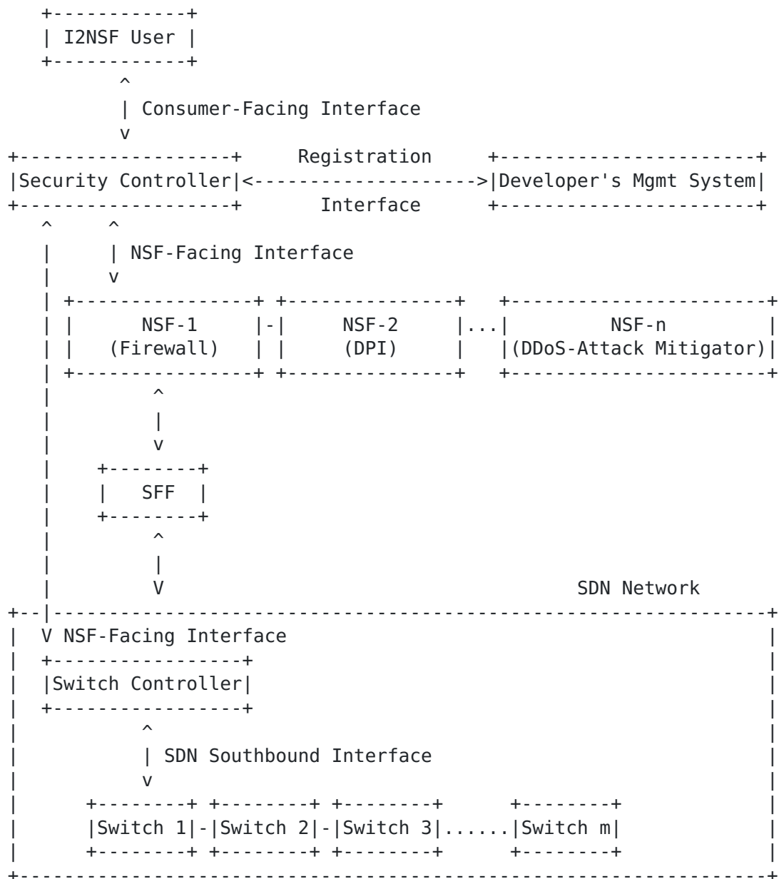
Figure 2: An I2NSF Framework with SDN Network
