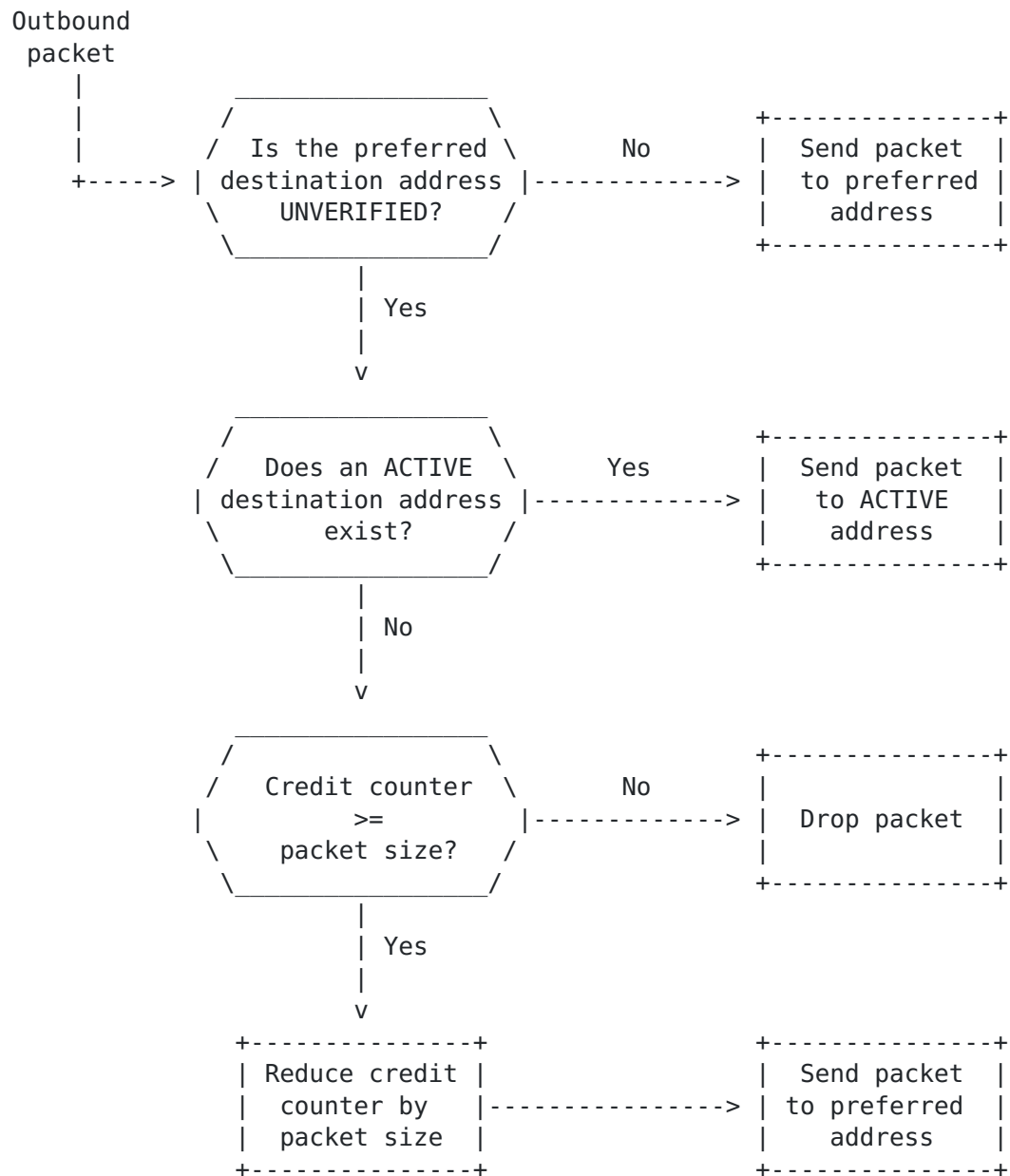
Figure 9: Sending Packets with Credit-Based Authorization
