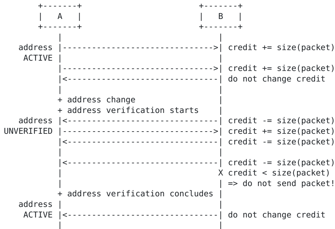
Figure 5: Readdressing Scenario
