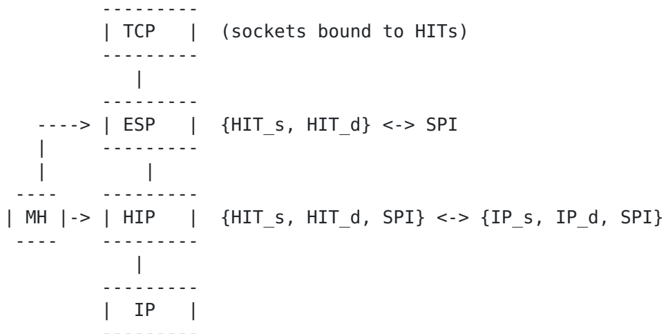
Figure 2: Architecture for HIP Host Mobility (MH)
