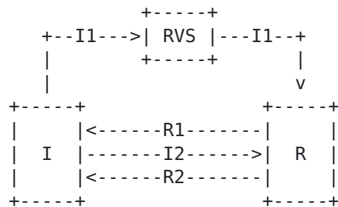
Figure 2: HIP base exchange with a rendezvous server.
