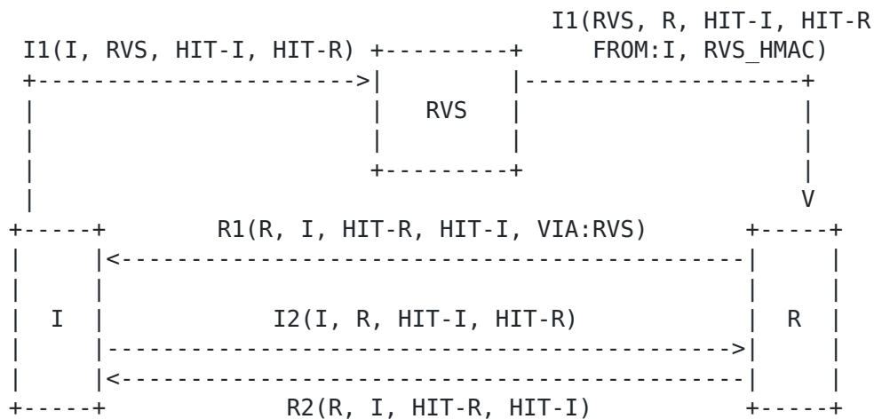
Rendezvous server rewriting IP addresses.
