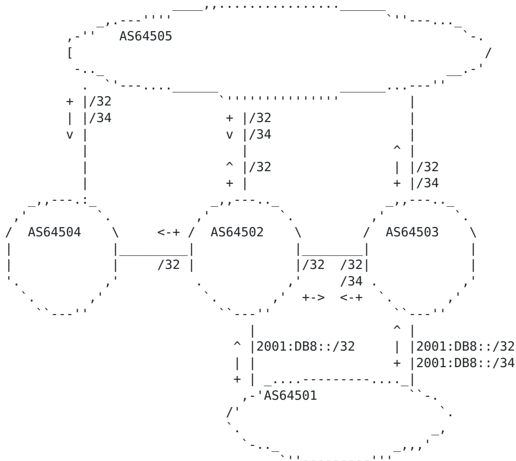
Figure 2: Unexpected traffic flows due to local filtering
