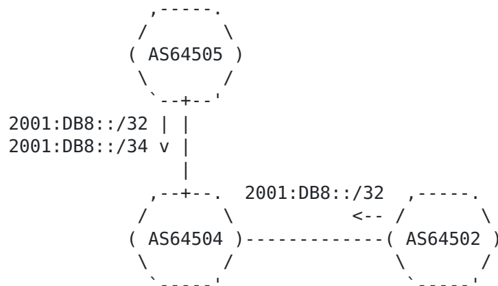
Figure 1: Local Filtering
