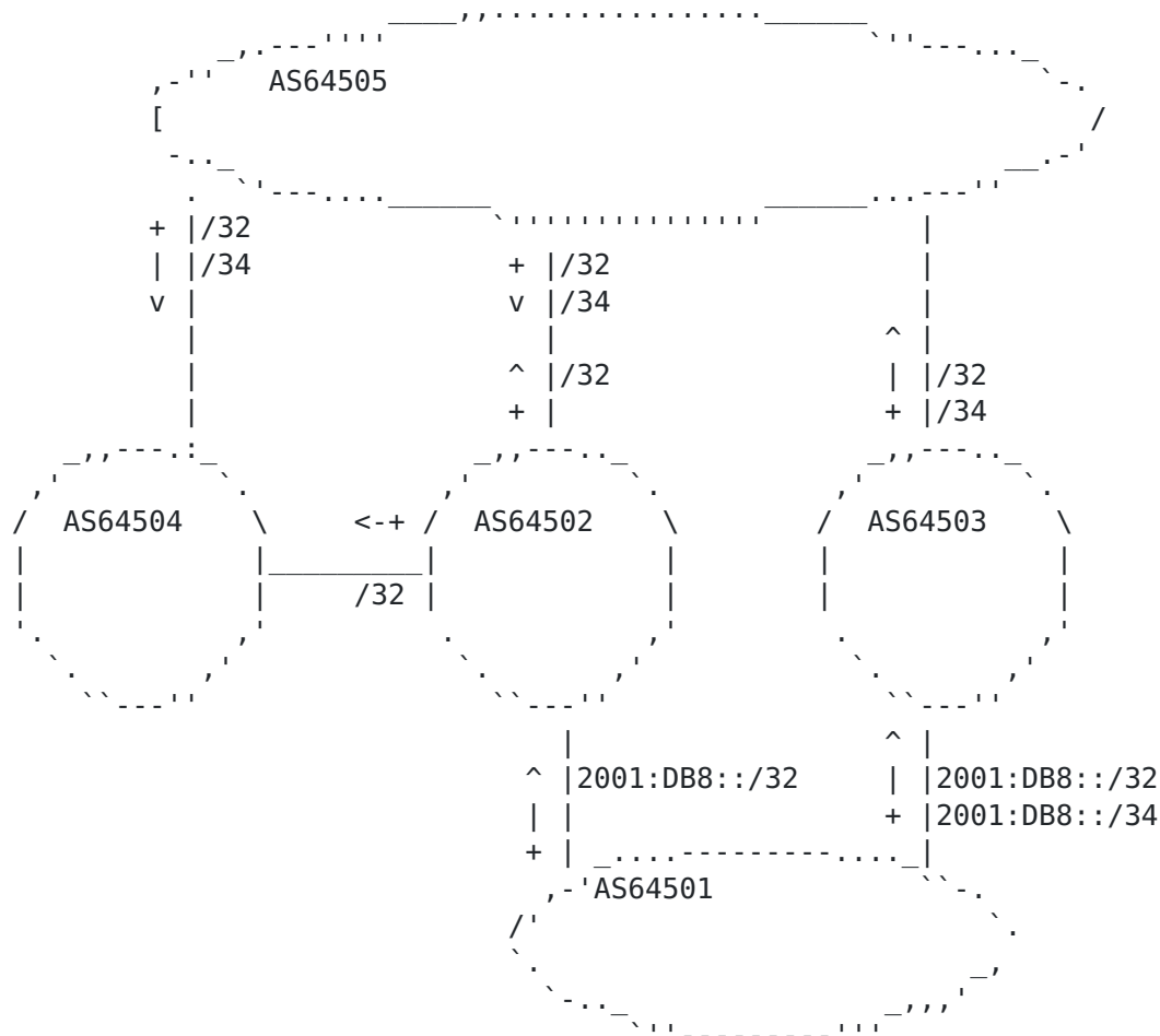
Figure 5: Traffic Engineering of unexpected traffic flows - Base example
