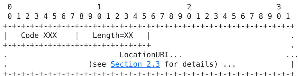
Figure 1. IPv4 Fields for this LocationURI Option
