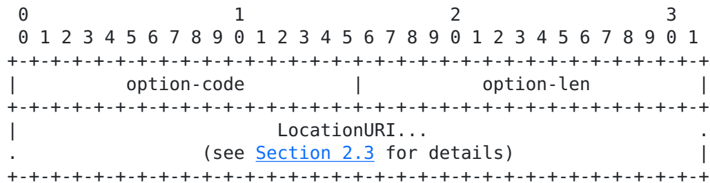
Figure 2. IPv6 fields of this LocationURI Option
