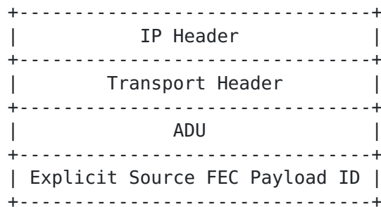
Figure 4: Structure of a FEC Source Packet with the Explicit Source FEC Payload ID.
