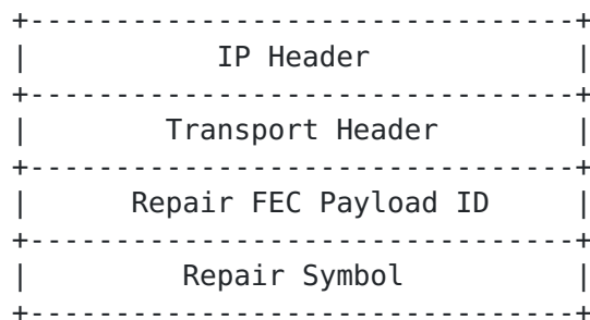
Figure 7: Structure of a FEC Repair Packet with the Repair FEC Payload ID.
