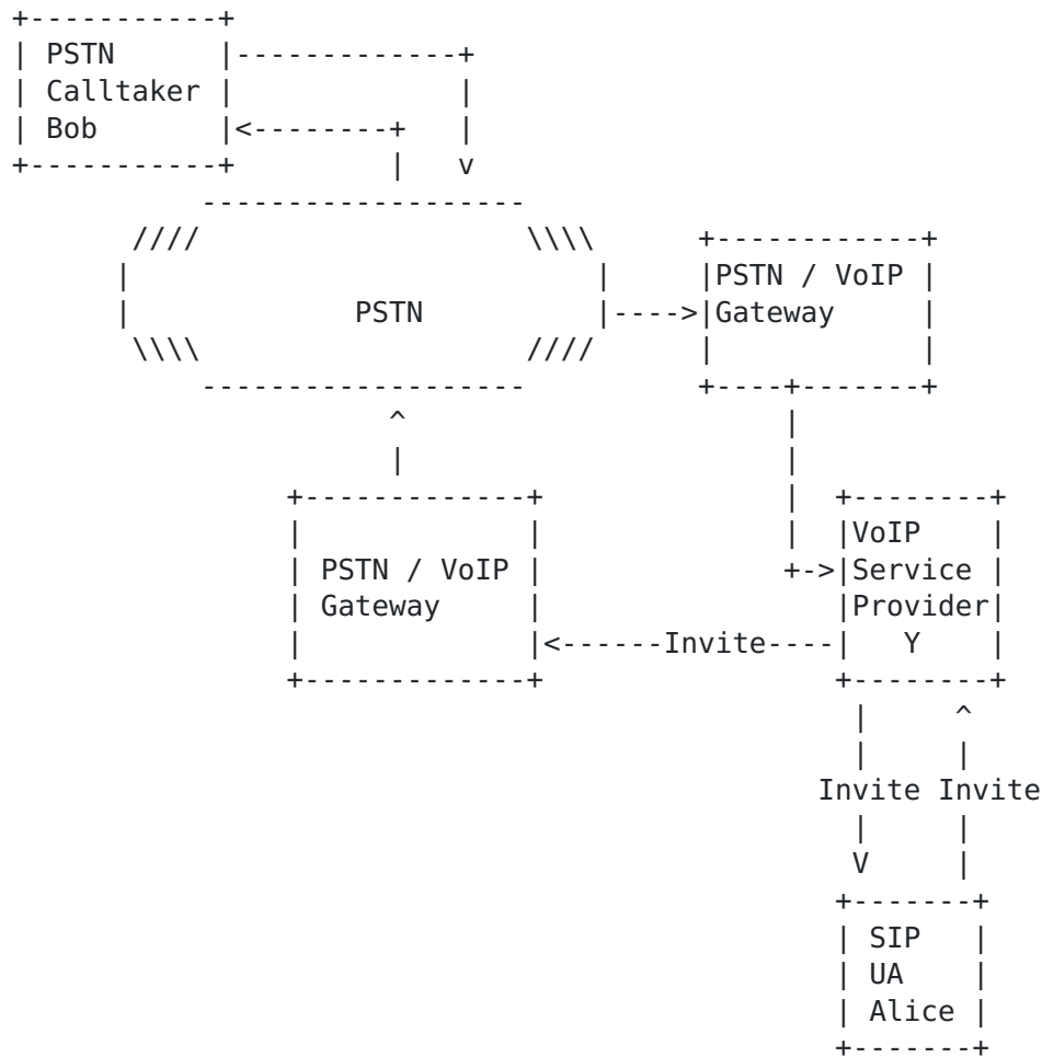
Figure 5: Example for PSTN Interworking.
