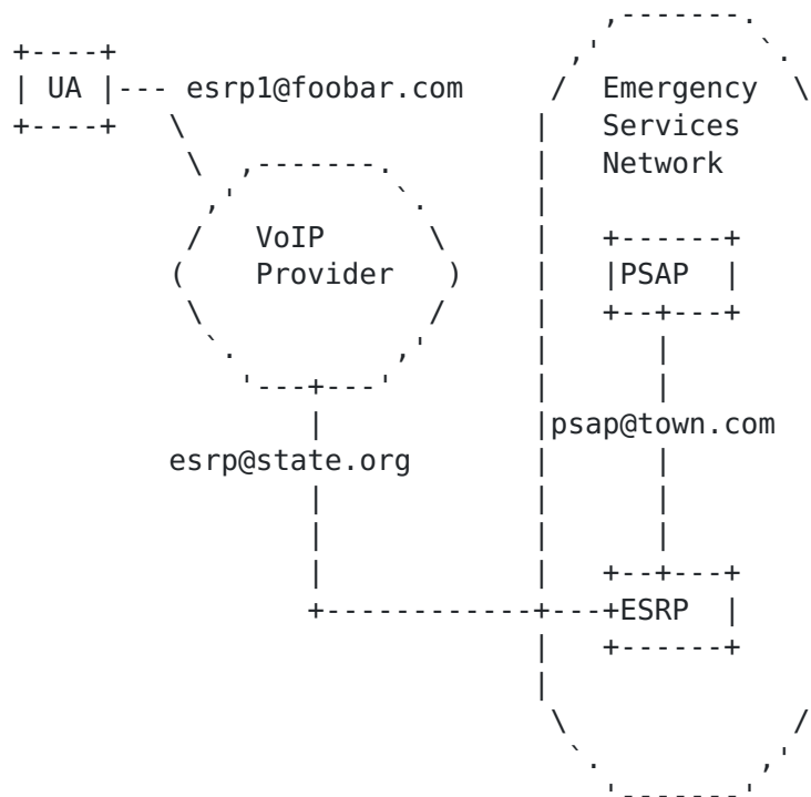
Figure 2: Example for Multi-Stage Routing.
