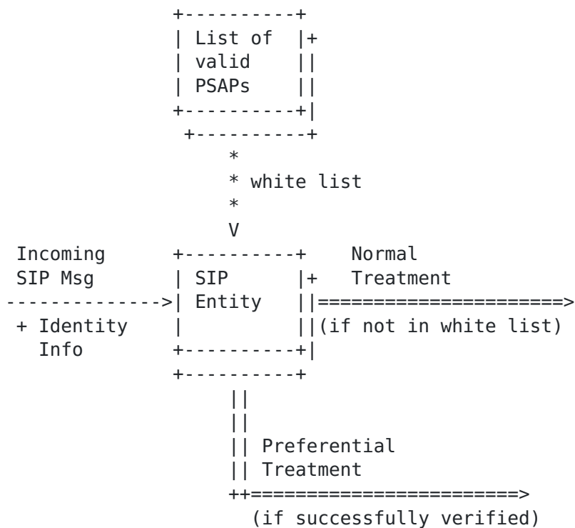
Figure 7: Identity-based Authorization
