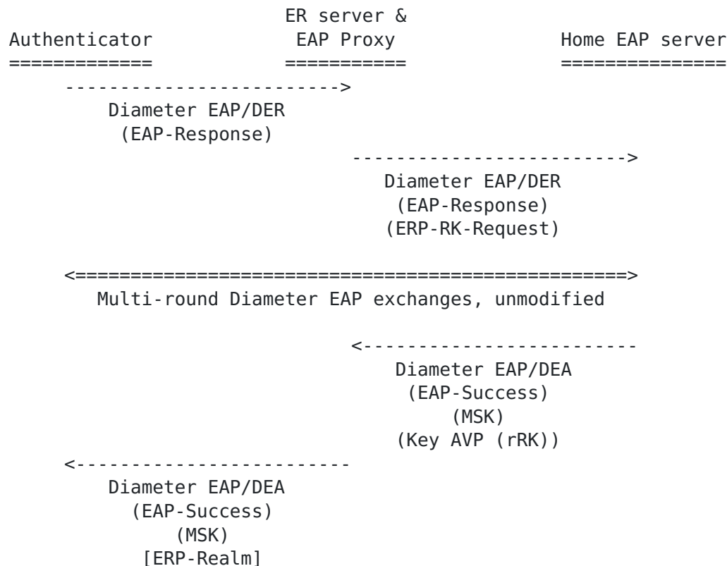
Figure 2: ERP Bootstrapping During Full EAP Authentication
