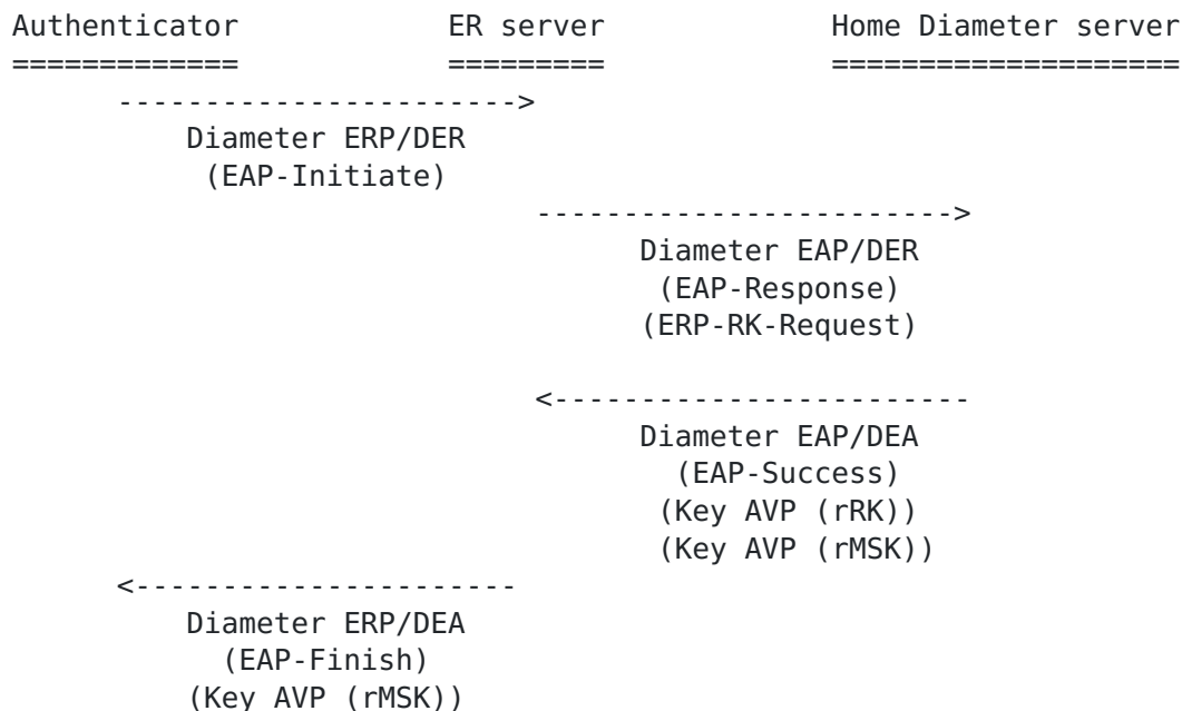
Figure 3: ERP Explicit Bootstrapping Message Flow
