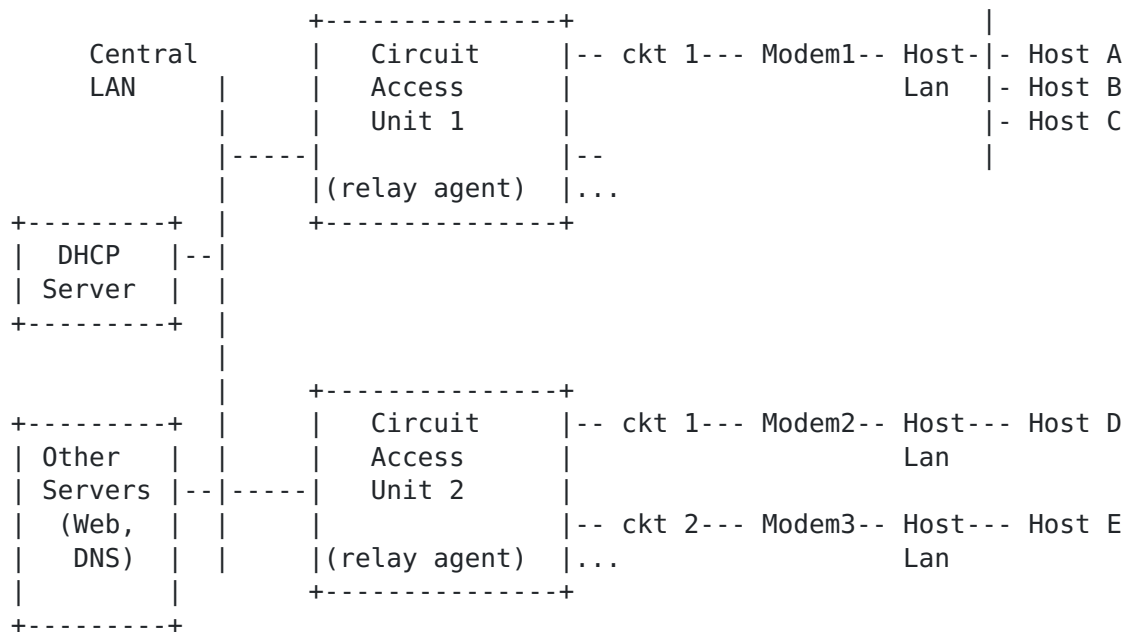
Figure 1: DHCP High Speed Circuit Access Model
