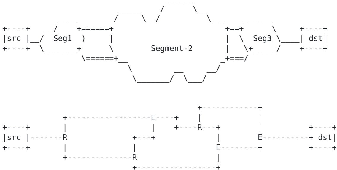
Figure 10: Optimal replication and elimination placement across technology segments example
