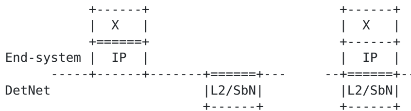
Figure 9: Encapsulation of DetNet Routing in simplified IP service L3 end-systems
