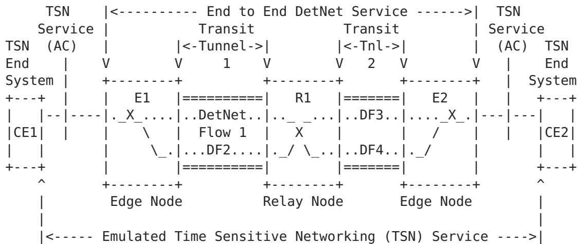
Figure 1: IEEE 802.1TSN over DetNet
