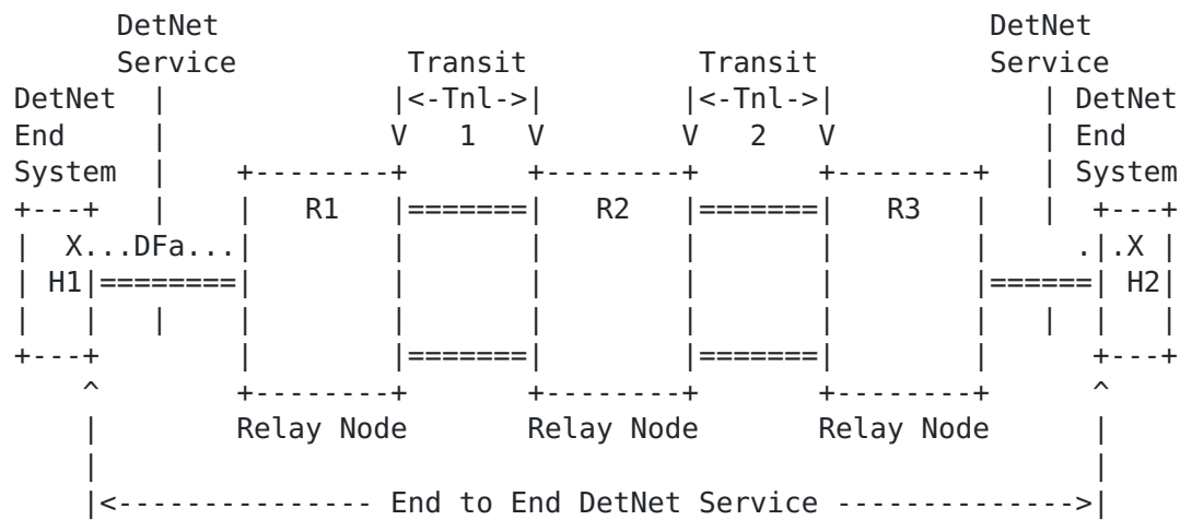
Figure 3: IP-Based Native DetNet
