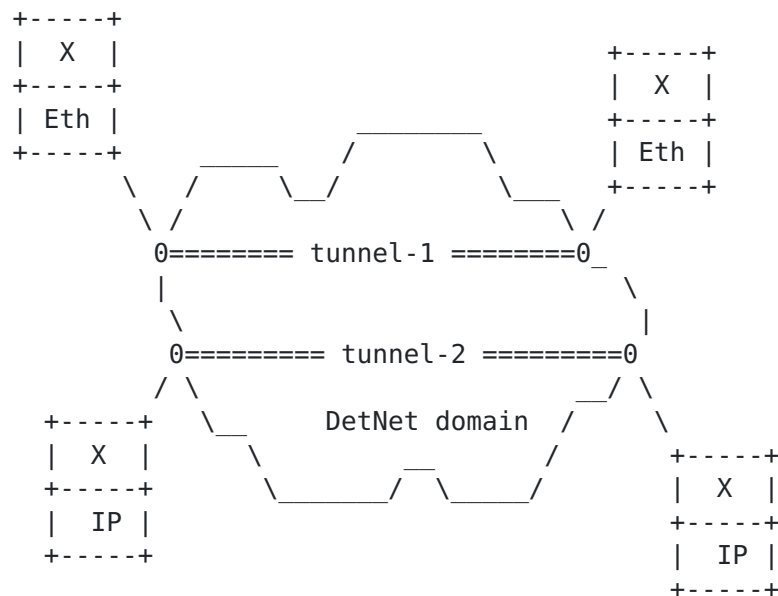
Figure 4: End-systems and the DetNet domain
