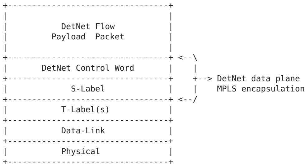
Figure 12: Encapsulation of a DetNet flow in an MPLS(-TP) PSN
