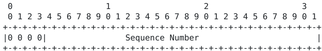
Figure 13: DetNet Control Word
