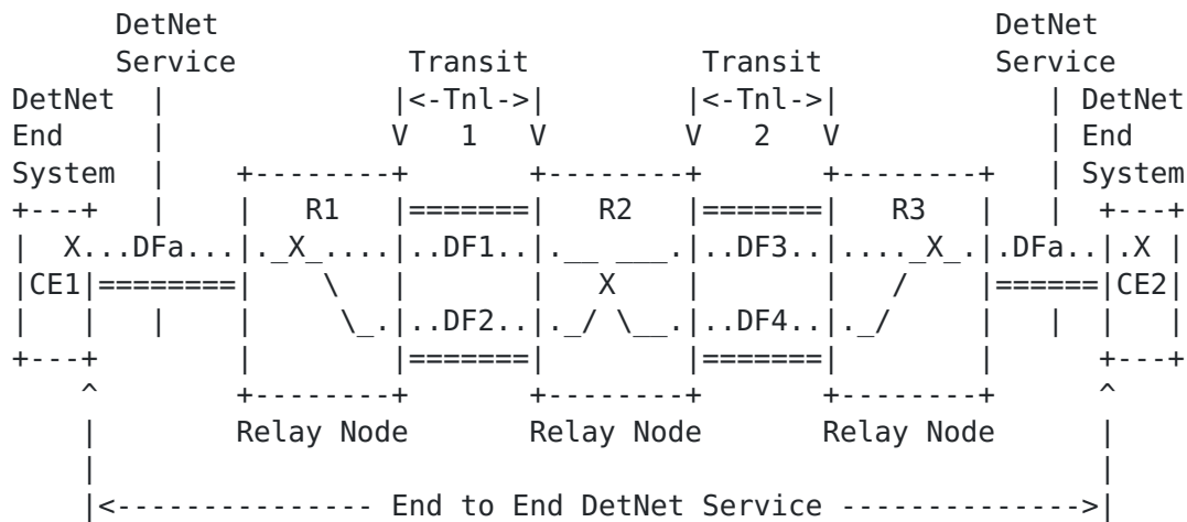
Figure 2: MPLS-Based Native DetNet
