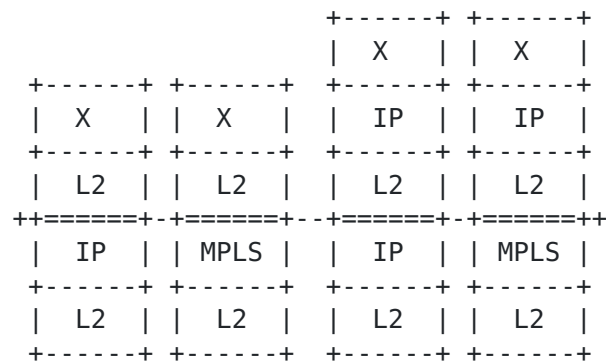
Figure 6: Encapsulation format for DetNet Bridging
