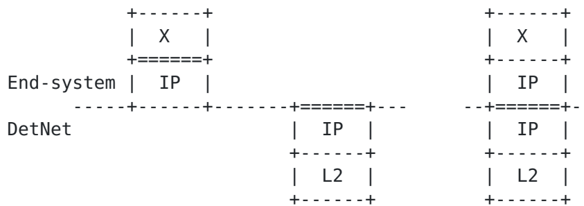
Figure 8: Encapsulation format for DetNet Routing in IP PSN for L3 end-systems
