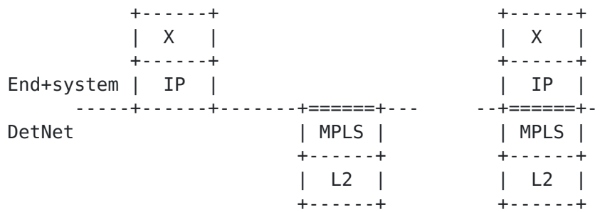
Figure 7: Encapsulation format for DetNet Routing in MPLS PSN for L3 end-systems
