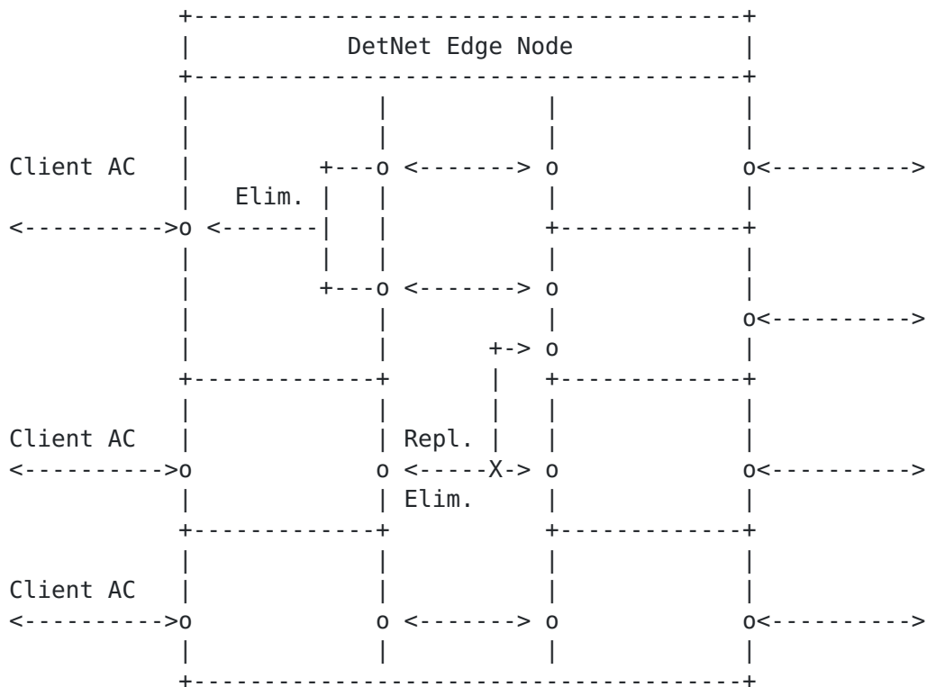
Figure 14: DetNet Edge Node processing
