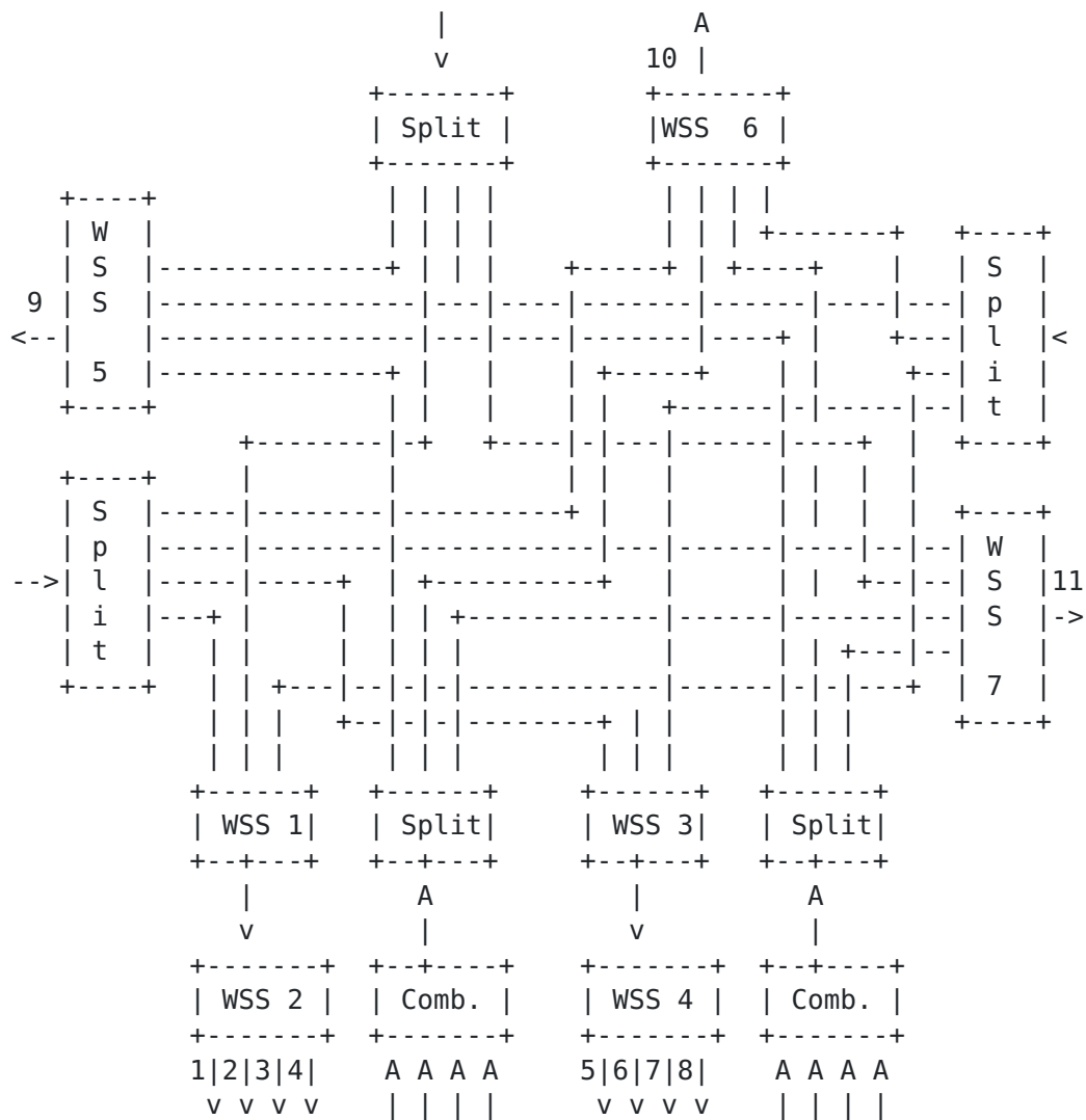
Figure 3 A ROADM composed from splitter, combiners, and WSSs.
