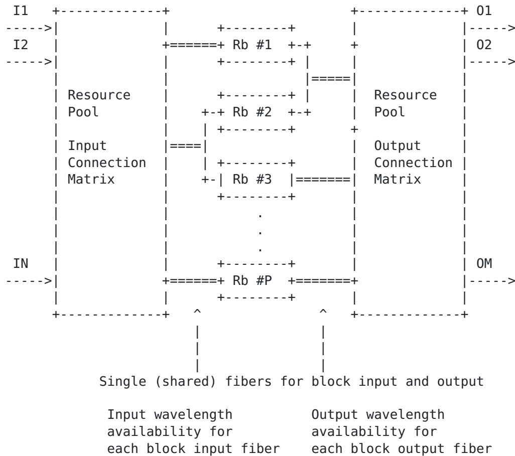
Figure 2 Schematic diagram of resource pool model with shared block accessibility.
