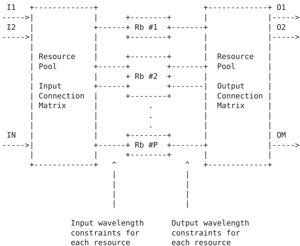
Figure 1 Schematic diagram of resource pool model.
