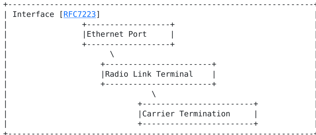
Figure 2: Relationship between interfaces in a node
