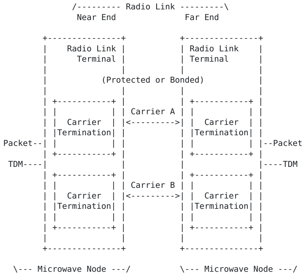
Figure 1. Radio Link Terminal and Carrier Termination
