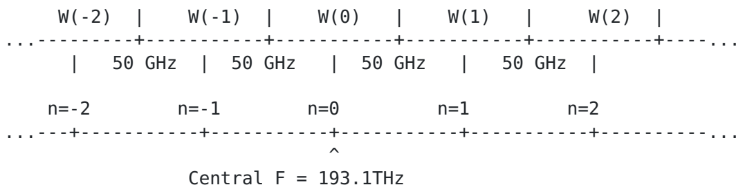
Figure 2 - A Link Supports Fixed Wavelengths with 50 GHz Channel Spacing
