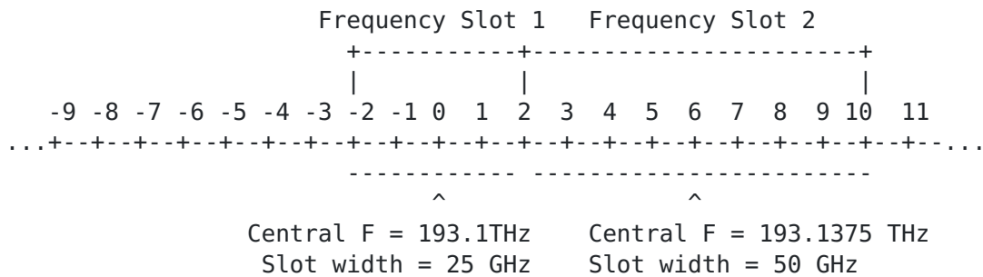
Figure 1 - Two Frequency Slots on a Link
