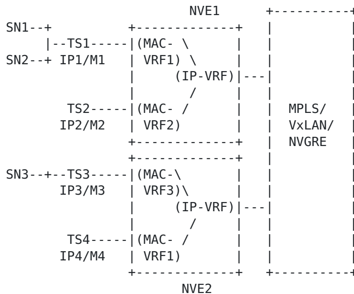
Figure 7: IRB forwarding on NVEs for subnets behind TSes
