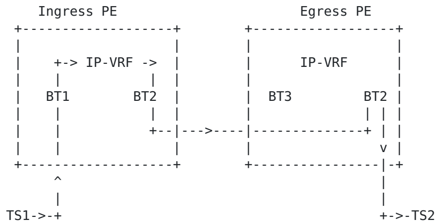
Figure 3: Asymmetric IRB
