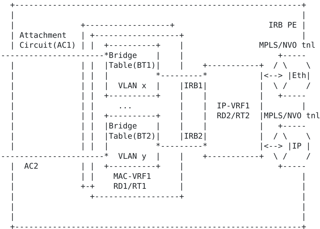
Figure 1: EVPN IRB PE Model
