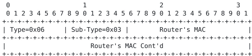
Figure 5: Router's MAC Extended Community
