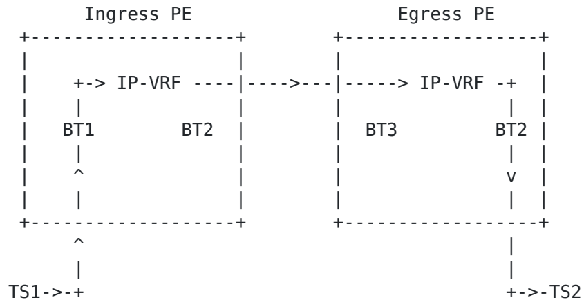
Figure 2: Symmetric IRB
