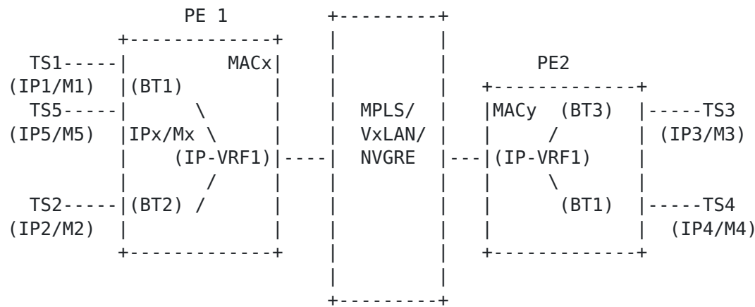
Figure 4: IRB forwarding
