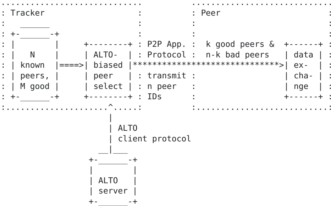
Figure 3: Tracker-based P2P Application with ALT0 client in tracker
