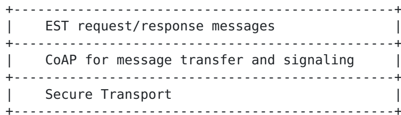
Figure 1: EST-coaps protocol layers
