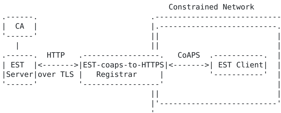
Figure 4: EST-coaps-to-HTTPS Registrar at the CoAP boundary.
