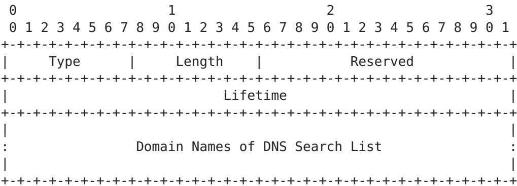
Figure 2: DNS Search List (DNSSL) Option Format
