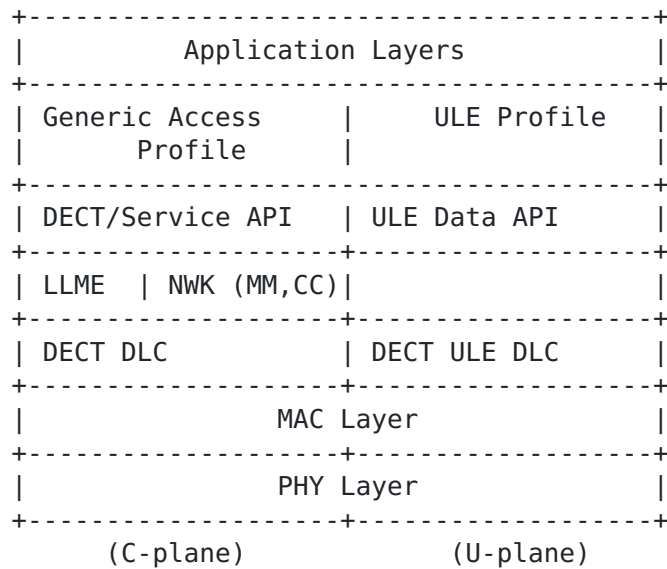
Figure 1: DECT ULE Protocol Stack
