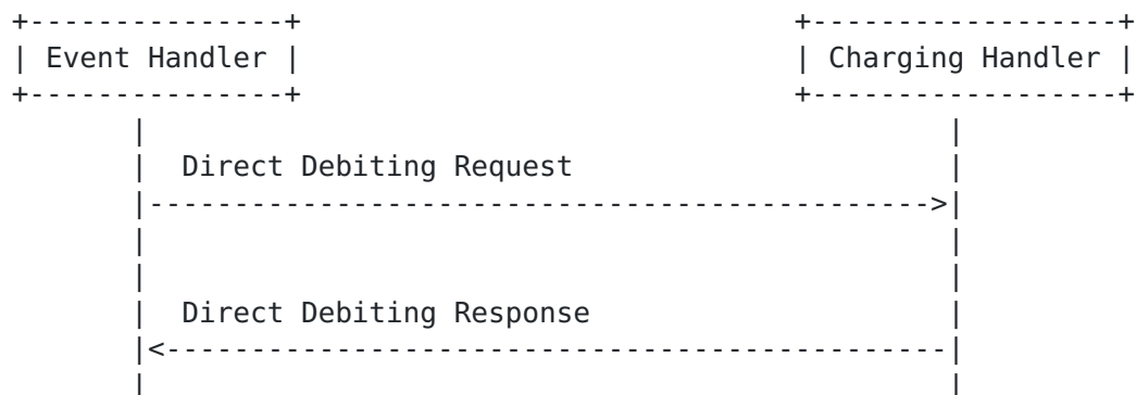
Figure 5: Direct Debiting Message Flow: Successful Case
