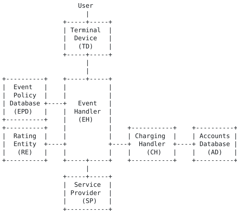
Figure 1: Framework with EH-RE Connection
