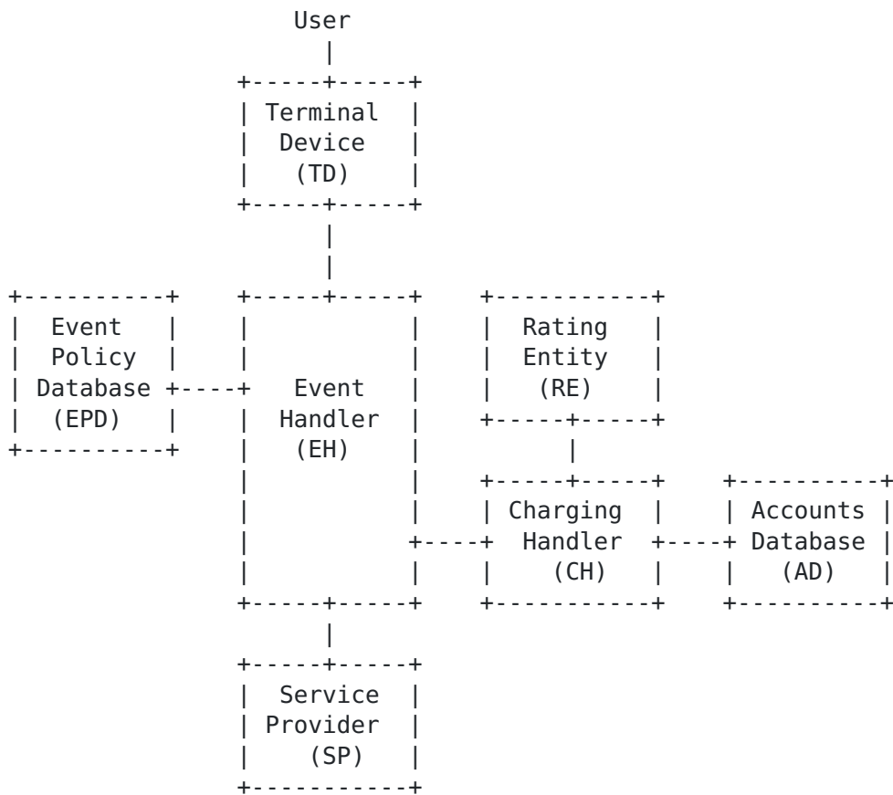
Figure 2: Framework with CH-RE Connection
