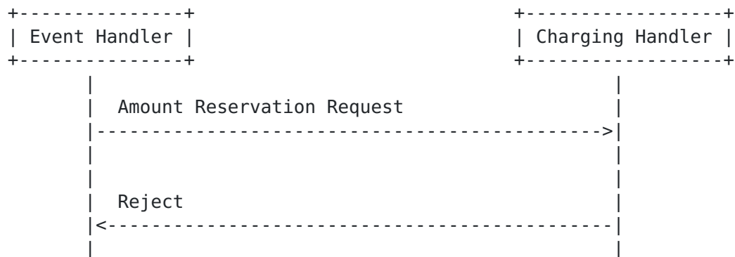
Figure 8: Amount Reservation Message Flow: Failure Case
