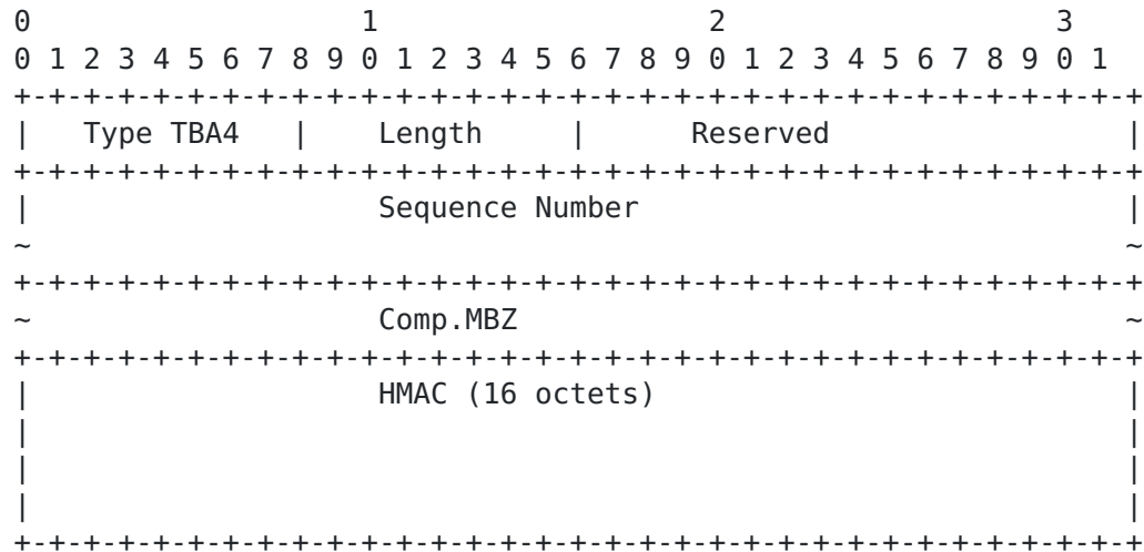
Figure 11: Sequence Number TLV - Authenticated Mode
