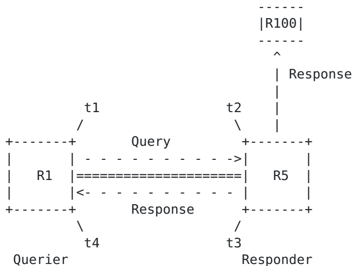
Reference Topology
