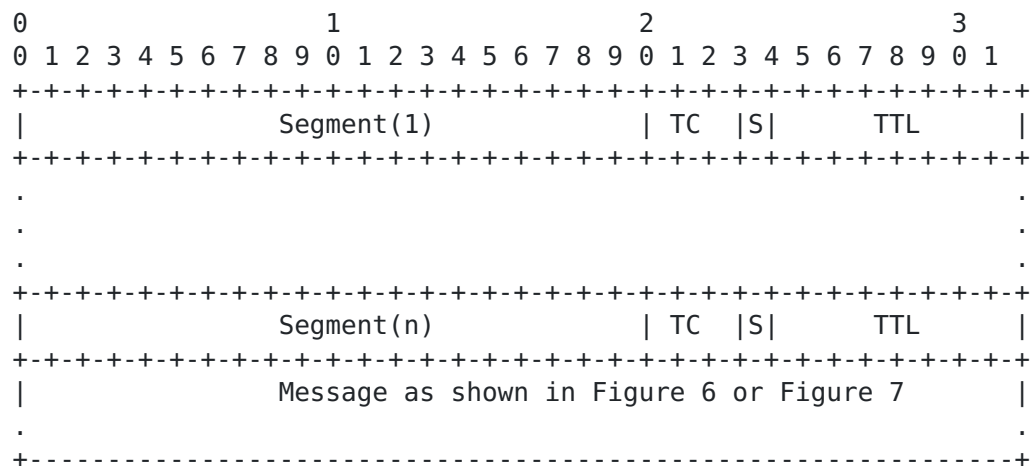
Figure 8: Example Probe Response Message for SR-MPLS Policy
