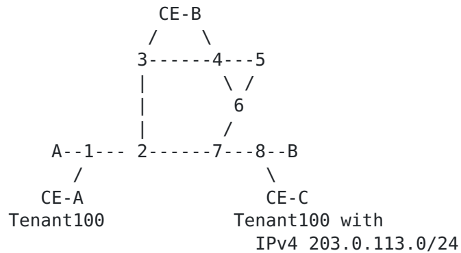
EVPN ESI filtering - Reference topology
