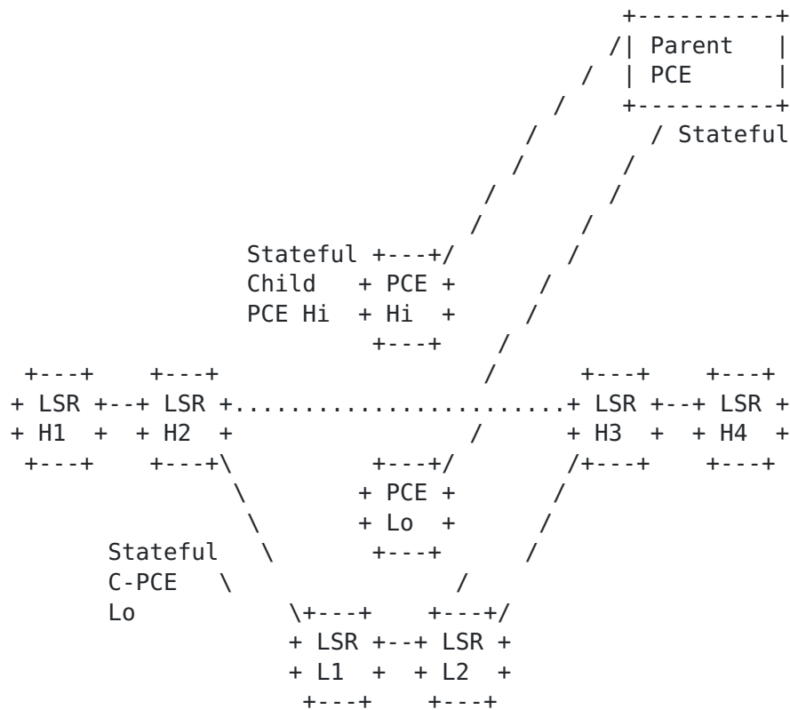
Figure 2: Sample Inter-Layer Topology
