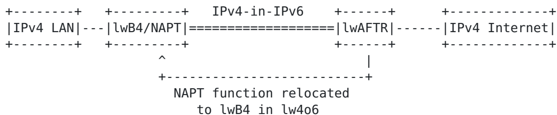
Figure 1 Lightweight 4over6 Data Plane Overview
