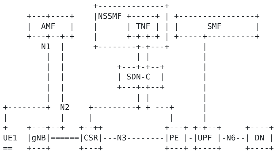
Figure 3: SSC Model with integrated Transport Slice Function
