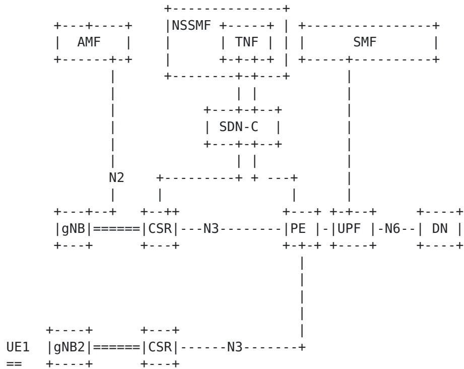
Figure 4: SSC Model with integrated Transport Slice Function
