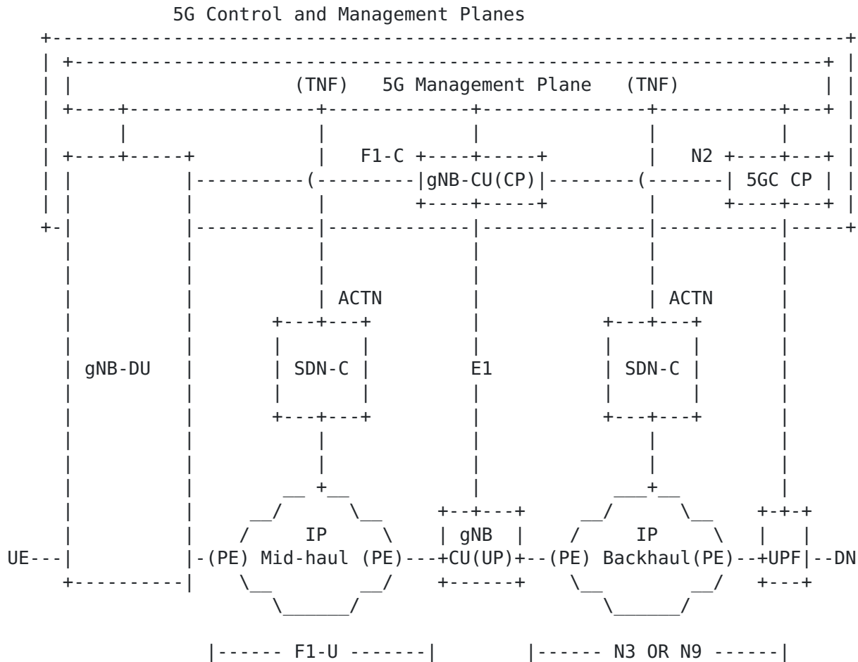
Figure 1: Backhaul and Mid-haul Transport Network for 5G
