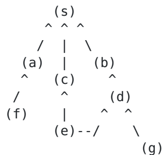
Figure 1: RPL DODAG
