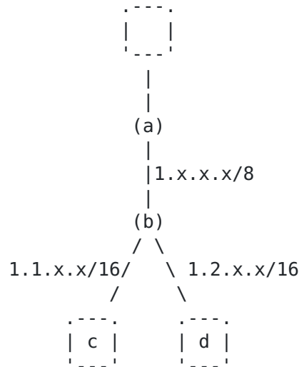
Figure 2: Address Hierarchies
