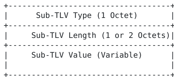
Figure 1: Geneve tunnel option types sub-TLV
