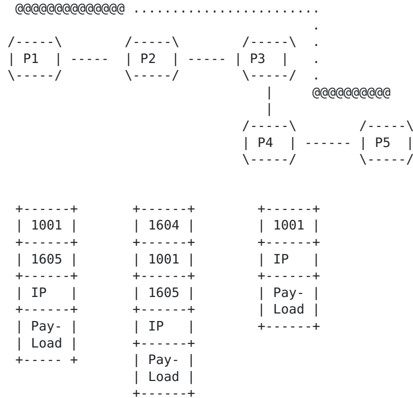
Figure 5: Extending network slice over slice policy incapable device(s).
