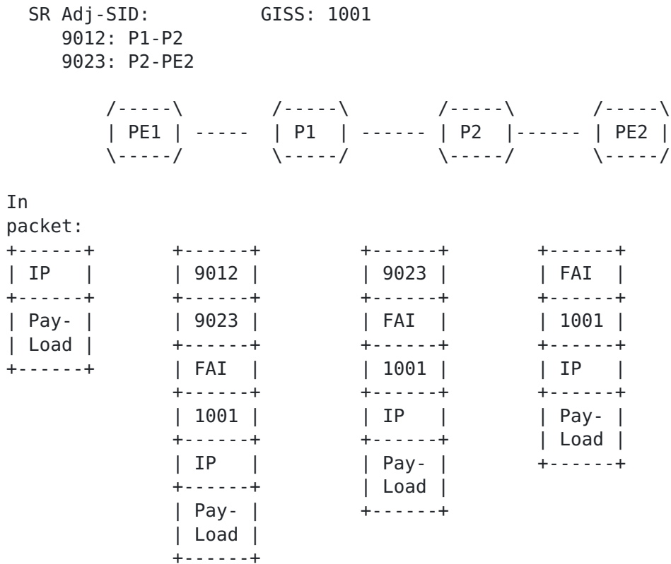
Figure 4: FAI and GISS label in the label stack.
