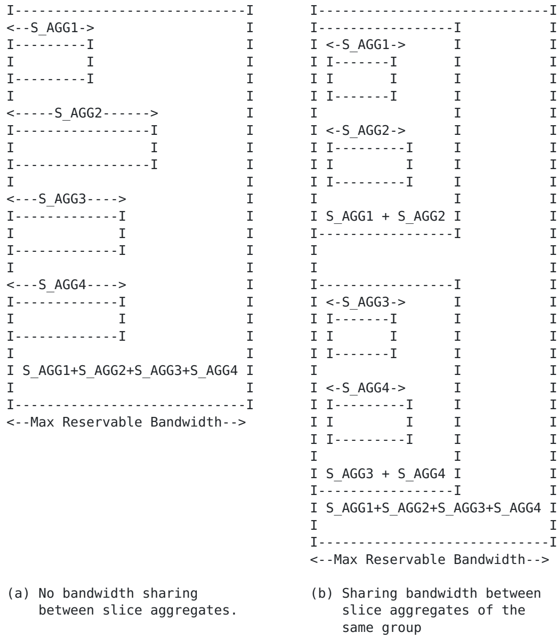
Figure 1: Bandwidth Isolation/Sharing.
