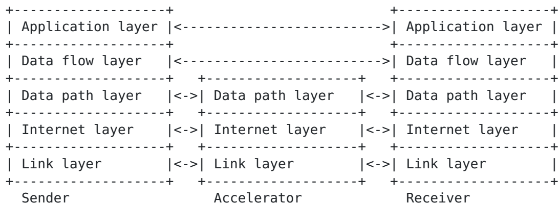
Figure 4: An example of a communication model for congestion control acceleration
