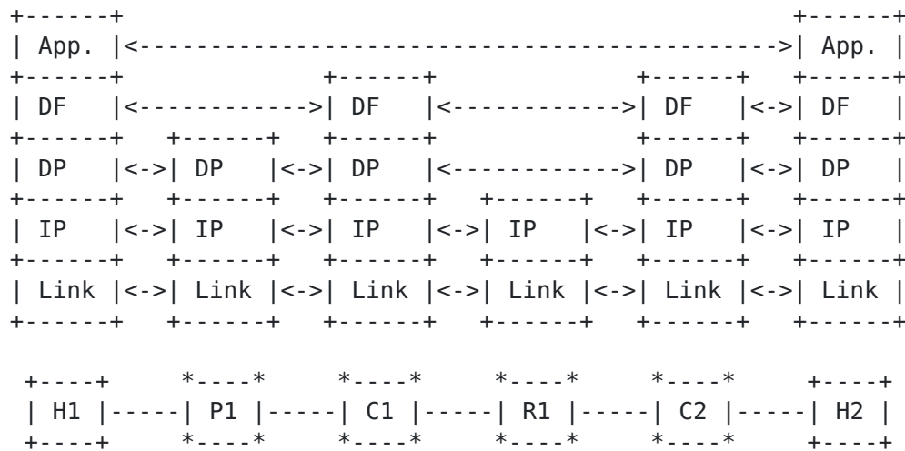
Figure 5: An example of communication model of in-network computing
