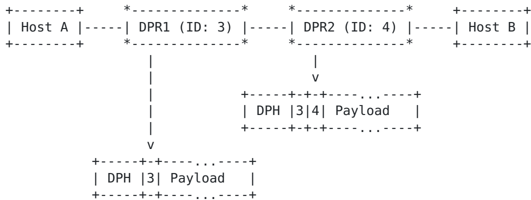
Figure 2: Appending data path router identifiers to distinguish the data path
