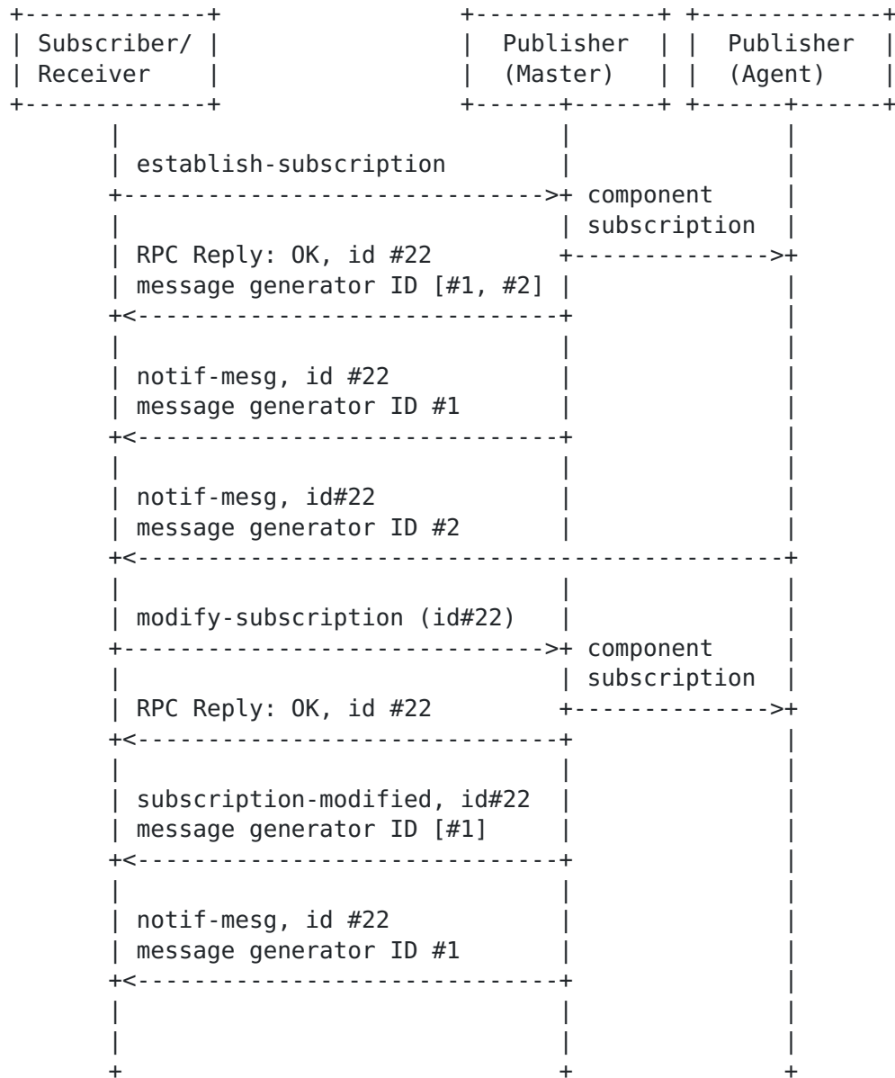
Fig. 3 Call Flow for Dynamic Subscription
