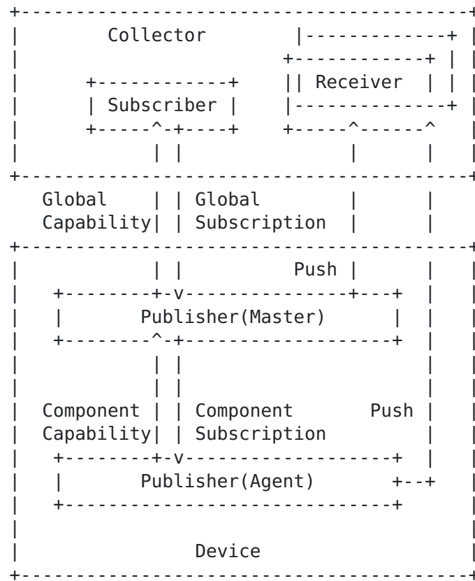
Fig. 2 The Distributed Data Export Framework
