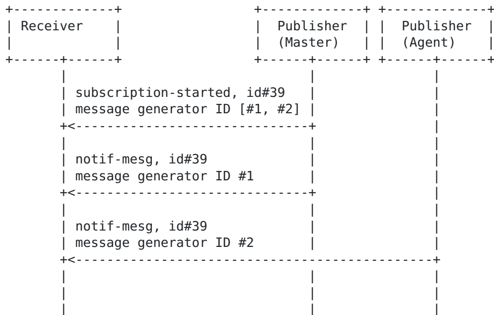
Fig. 8 Call Flow for Configured Subscription
