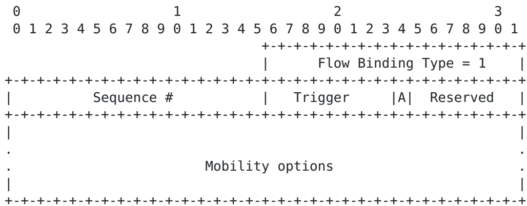
Figure 3: Flow Binding Indication Mobility Header Format
