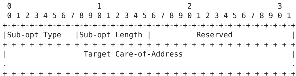
Figure 6: Target Care-of-Address Sub-option
