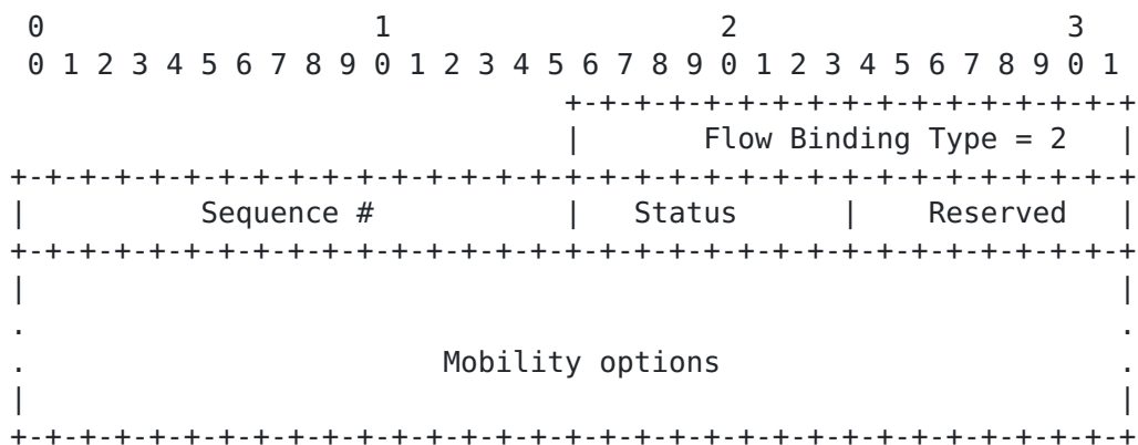
Figure 4: Flow Binding Acknowledgement Mobility Header Format
