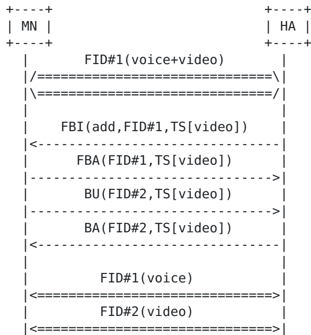
Figure 1: Example call flow for adding a flow binding
