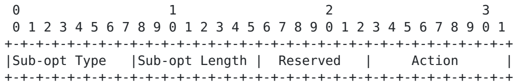
Figure 5: Flow binding action sub-option
