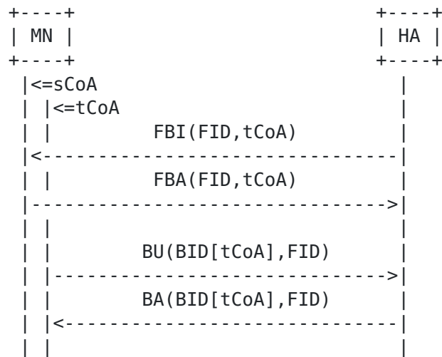
Figure 2: Example call flow for moving a flow binding
