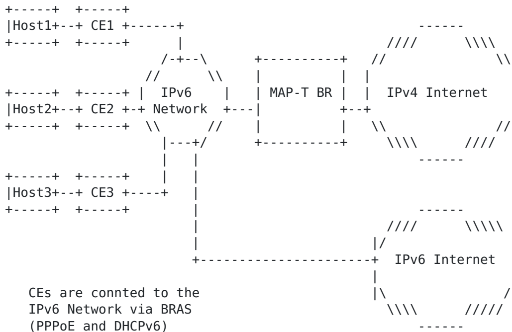
Figure 1: MAP-T Lab Test
