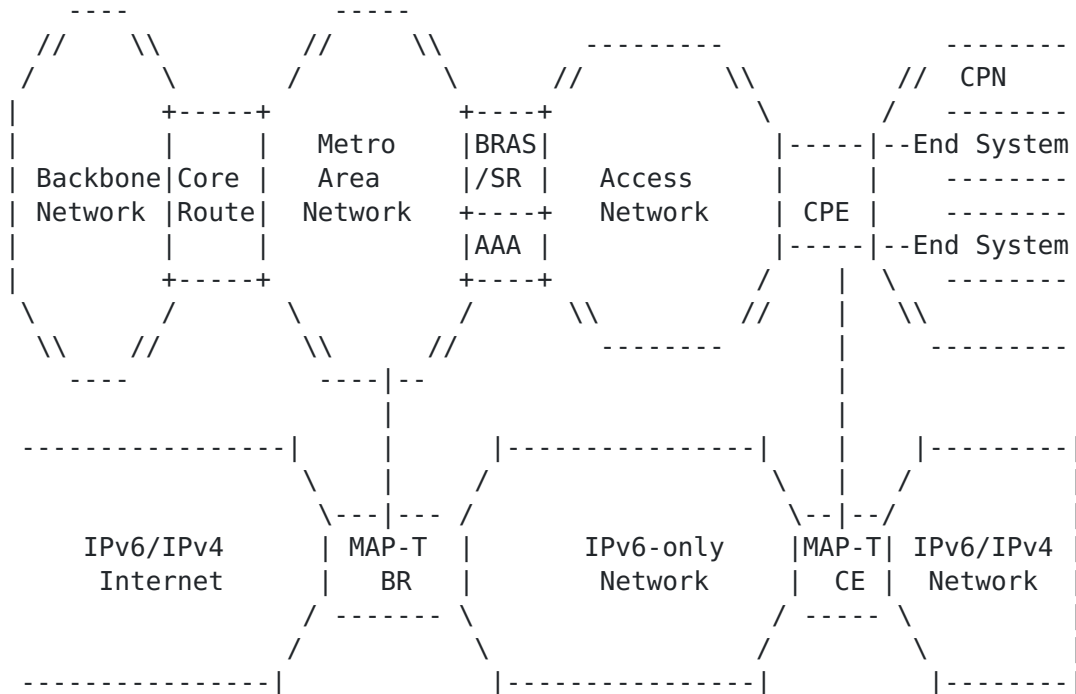
Figure 2: MAP-T Field Trial
