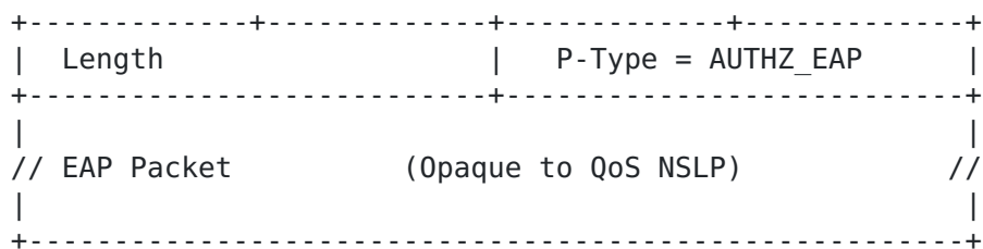
Figure 5: Format of EAP Policy Element
