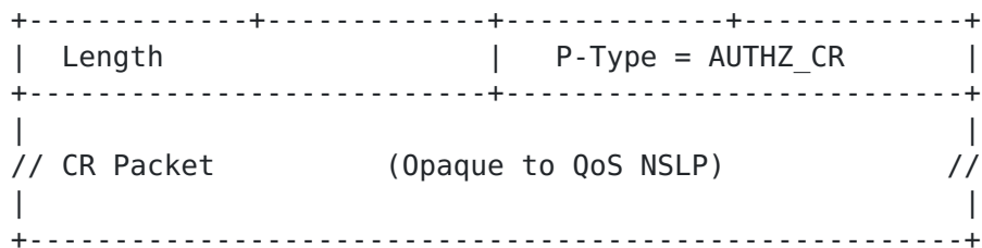
Figure 4: Format of CR Policy Element
