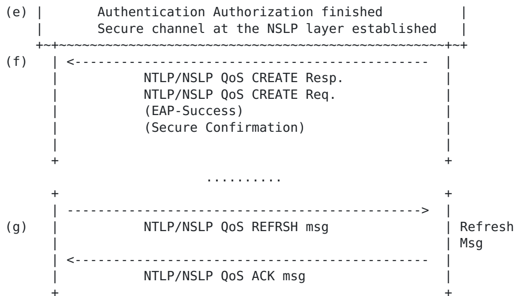
Figure 3: EAP based Auth/Authz exchange using EAP-AKA
