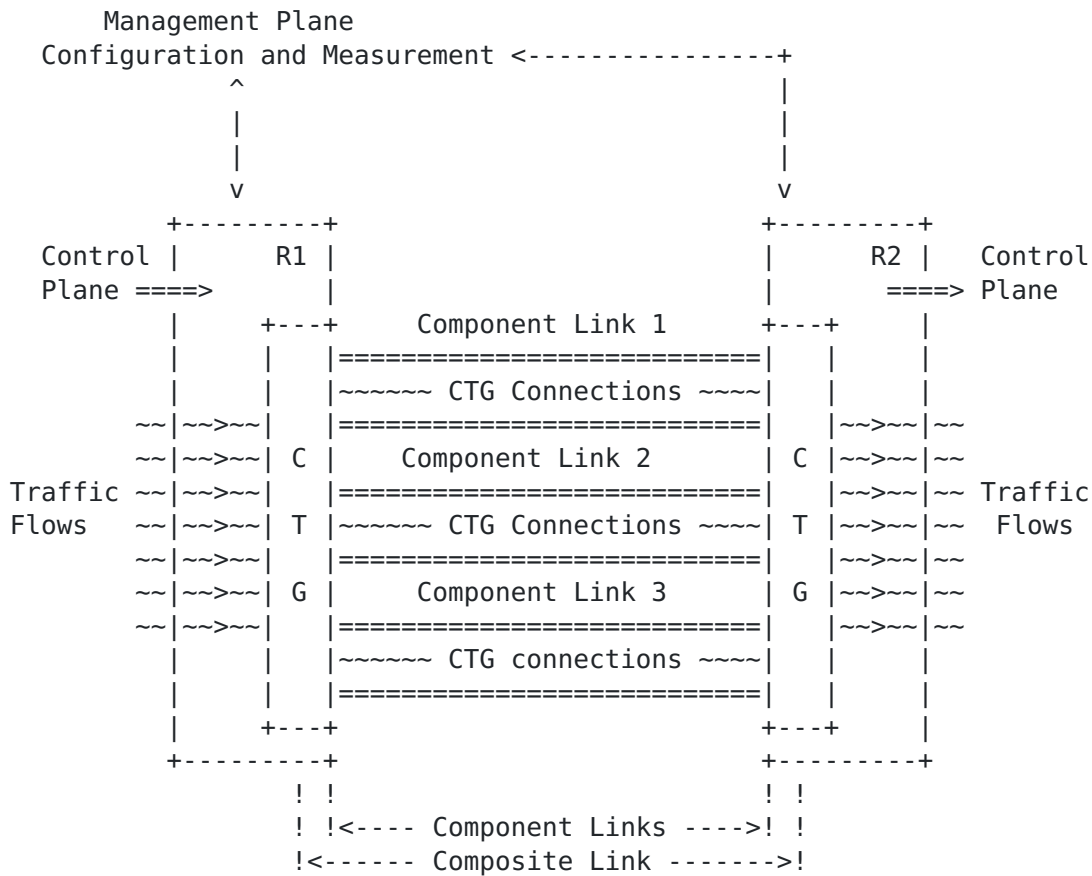
Figure 1: Composite Transport Group Architecture Model
