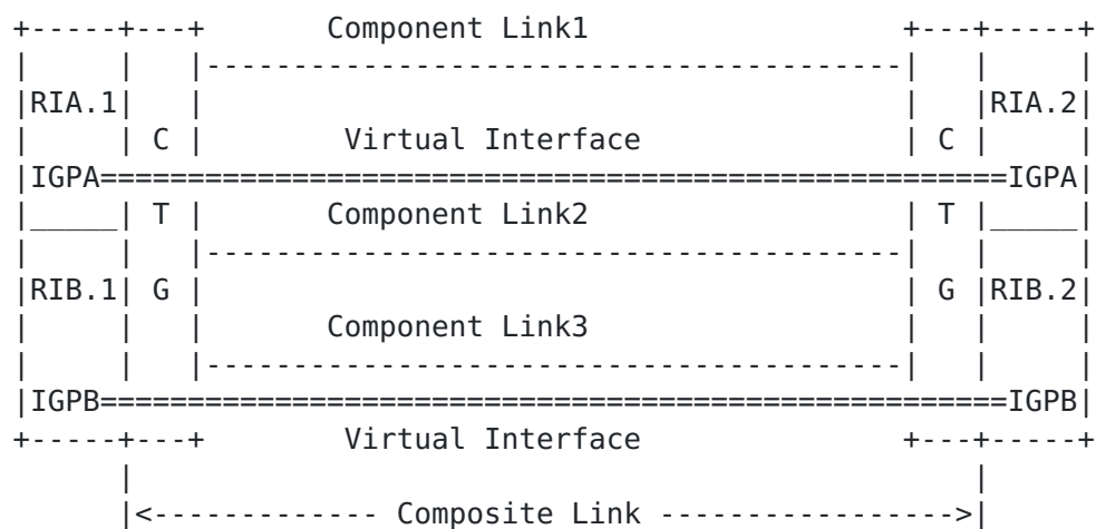
Figure 3: Routing Instances Sharing Composite Link
