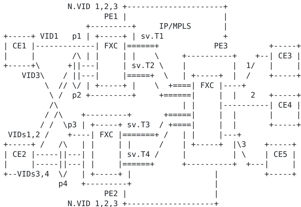
Figure 2 Default Flexible Xconnect
