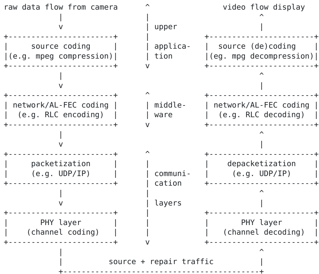
Figure 2: Example of end-to-end flow manipulation with Network Coding between the application and UDP layers (as with RMT or FECFRAME architectures). Other architectures are possible, for instance with network coding below the transport layer in order to allow re-coding within the network.
