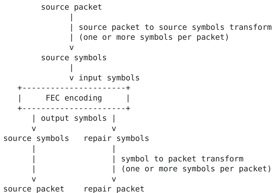
Figure 1: Packet and symbol relationships at a Coding Node.
