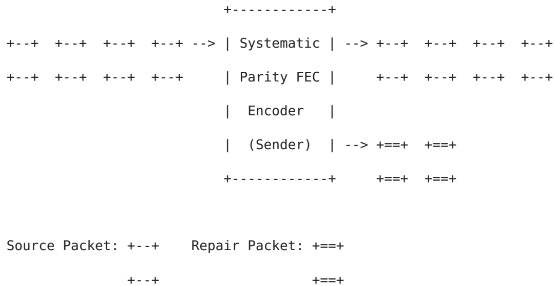
Figure 1: Block diagram for systematic parity FEC encoder
