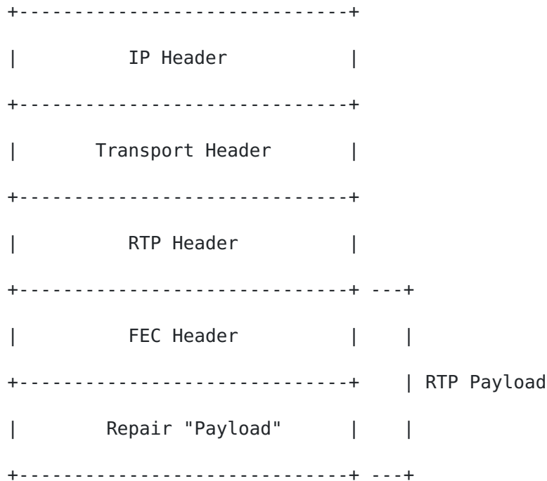
Figure 9: Format of FEC repair packets
