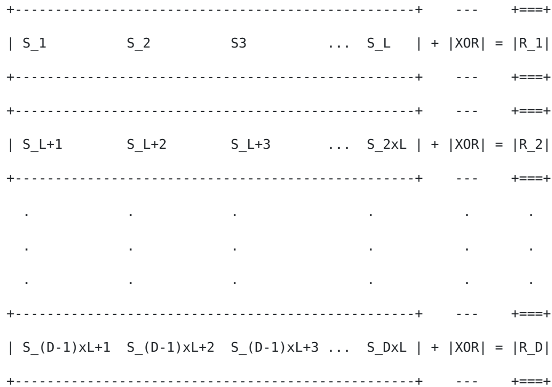
Figure 3: Generating non-interleaved (row) FEC repair packets
