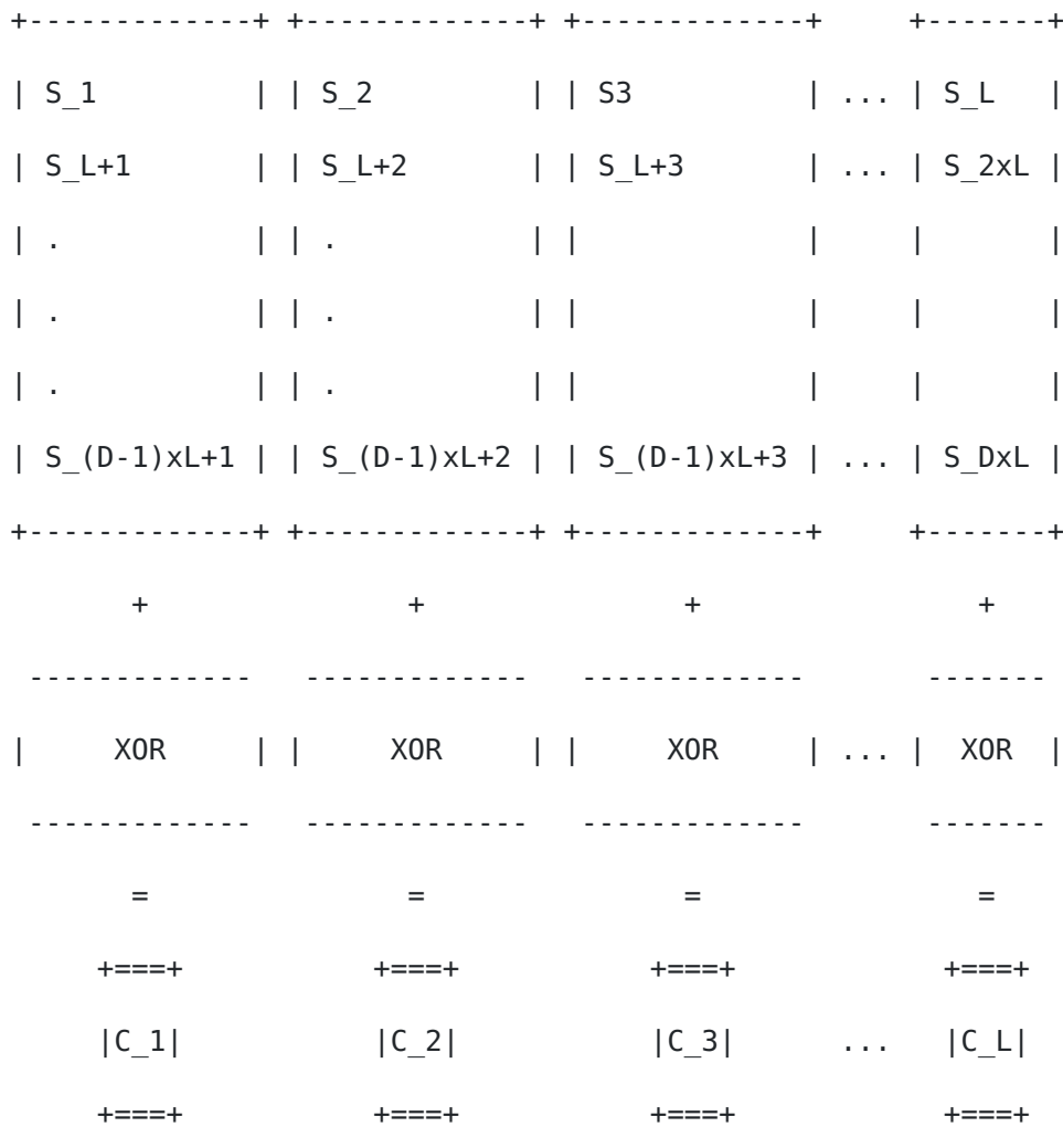
Figure 4: Generating interleaved (column) FEC repair packets
