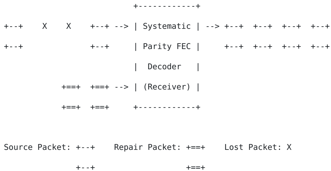
Figure 2: Block diagram for systematic parity FEC decoder
