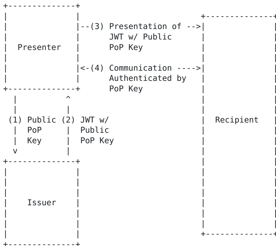
Figure 2: Proof-of-Possession with an Asymmetric Key
