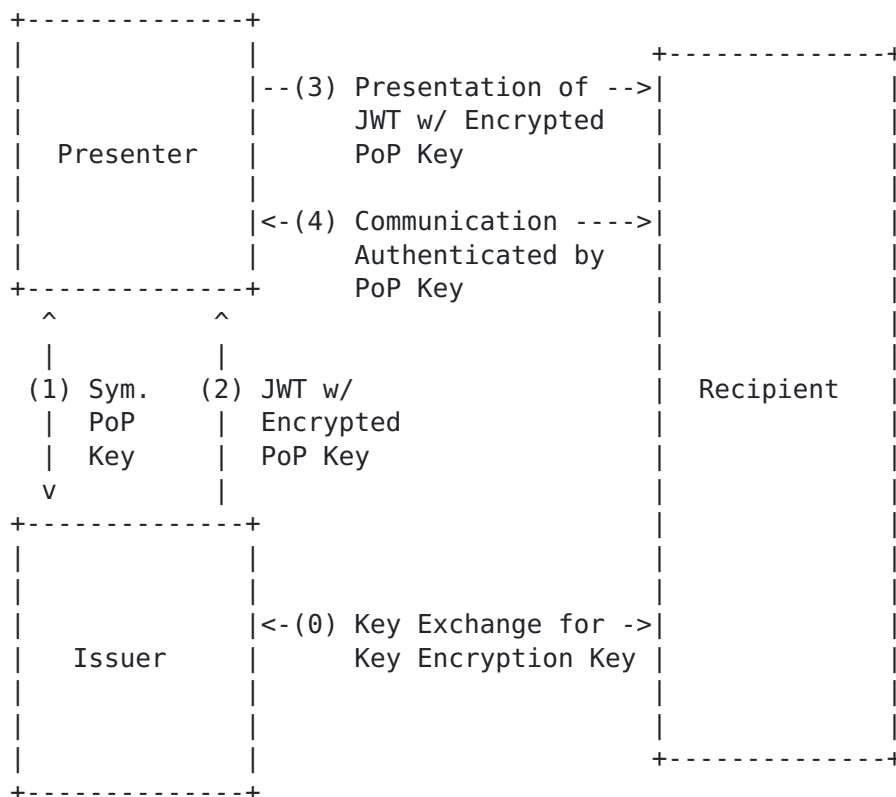
Figure 1: Proof-of-Possession with a Symmetric Key
