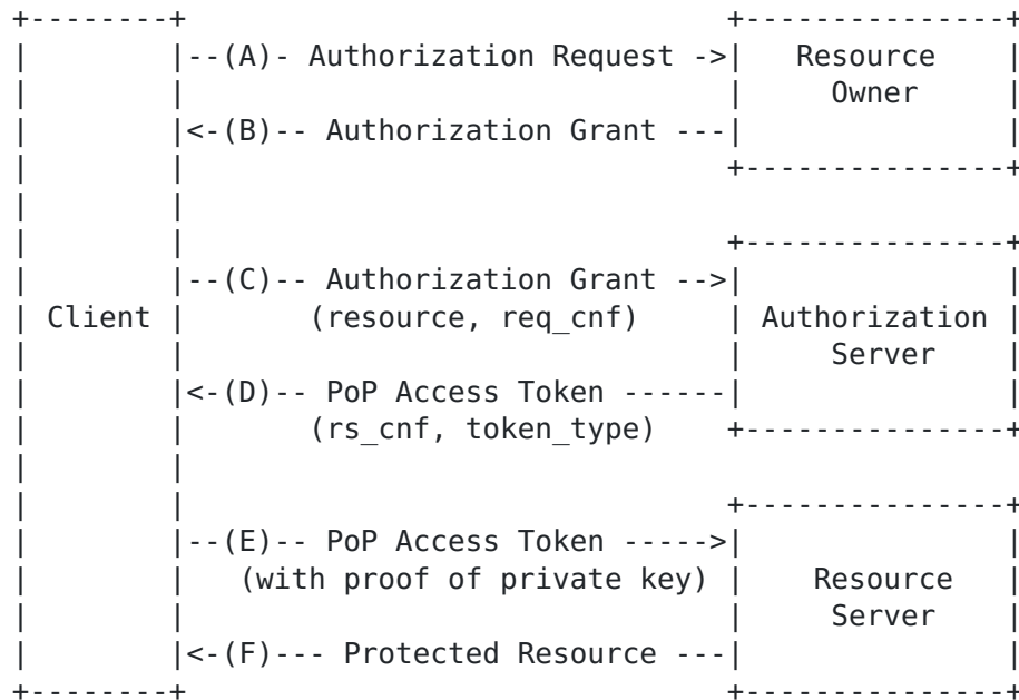
Figure 1: Augmented OAuth 2.0 Protocol Flow
