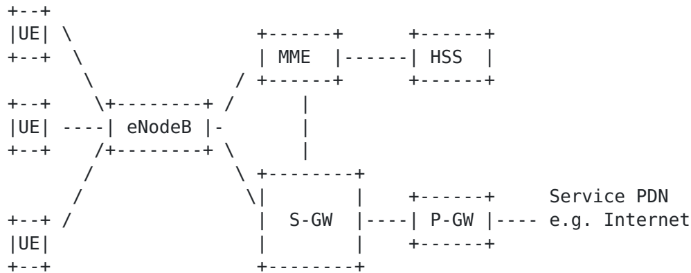
Figure 3: 3GPP network architecture
