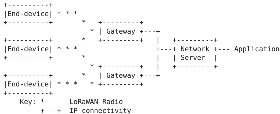
Figure 1: LoRaWAN architecture
