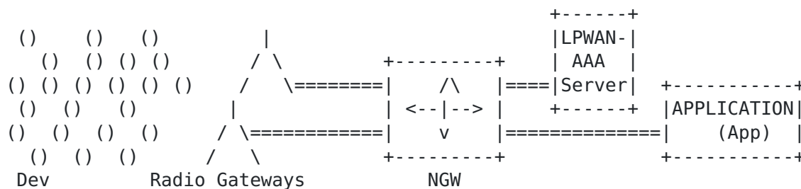
Figure 9: LPWAN Architecture
