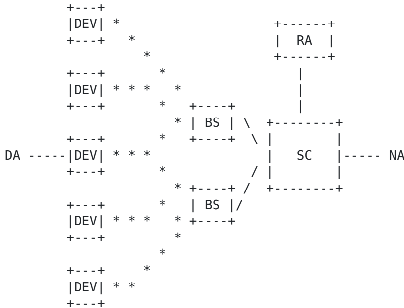
Figure 7: SIGFOX network architecture
