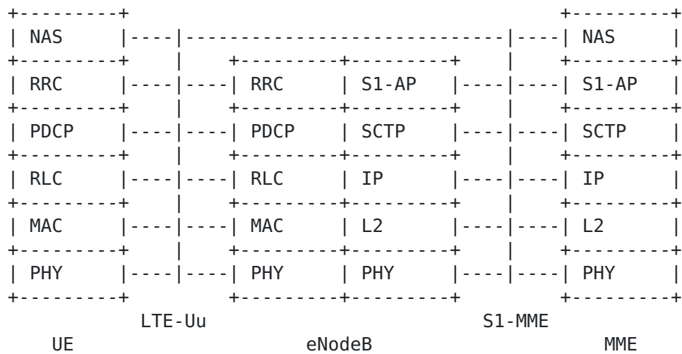
Figure 4: 3GPP radio protocol architecture for control plane
