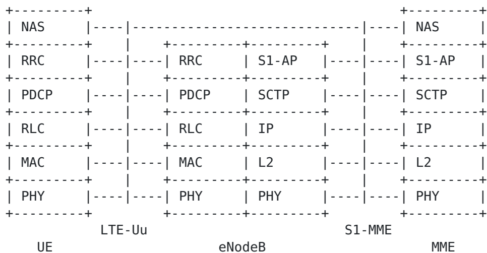
Figure 4: 3GPP radio protocol architecture
