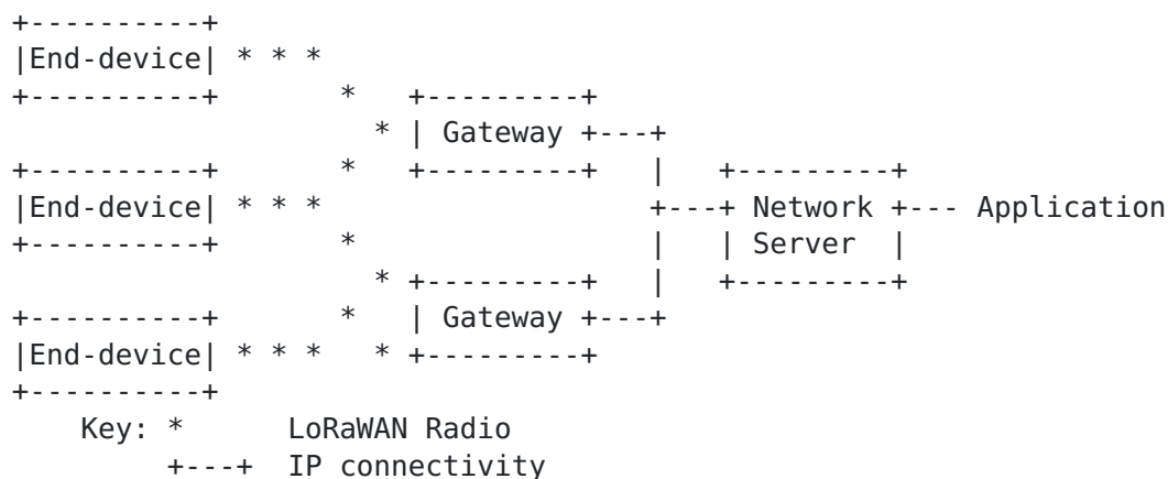
Figure 1: LoRaWAN architecture
