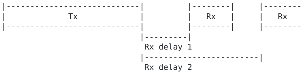
Figure 2: LoRaWAN Class A transmission and reception window
