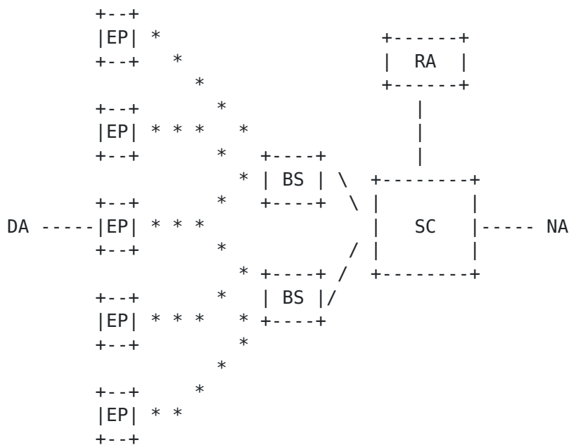
Figure 7: SIGFOX architecture
