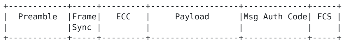
Figure 6: Downlink Frame Format
