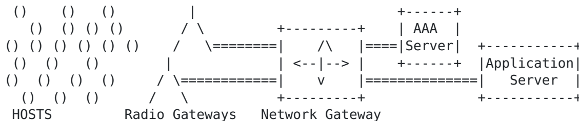
Figure 9: LPWAN Architecture
