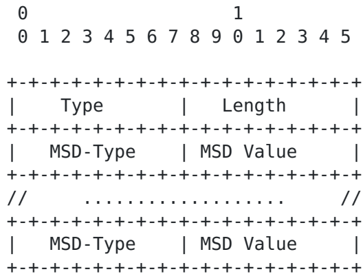
Figure 1: Node MSD Sub-TLV
