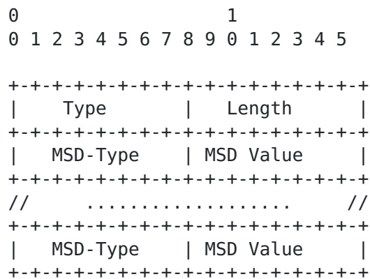
Figure 2: Link MSD Sub-TLV
