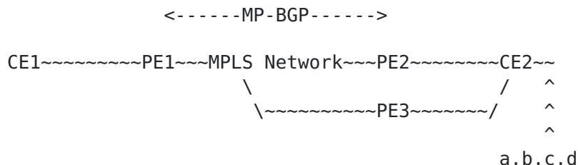
Figure 2 MPLS VPN Network - CE2 Dual-Homing
