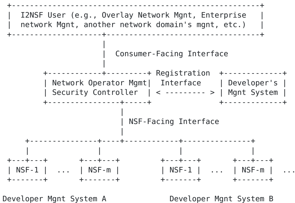
Figure 1: I2NSF Reference Model
