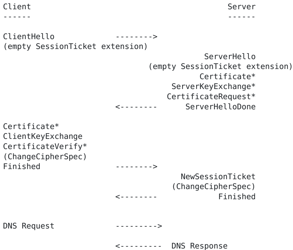
Figure 1: Message Flow for Full Handshake Issuing New Session Ticket
